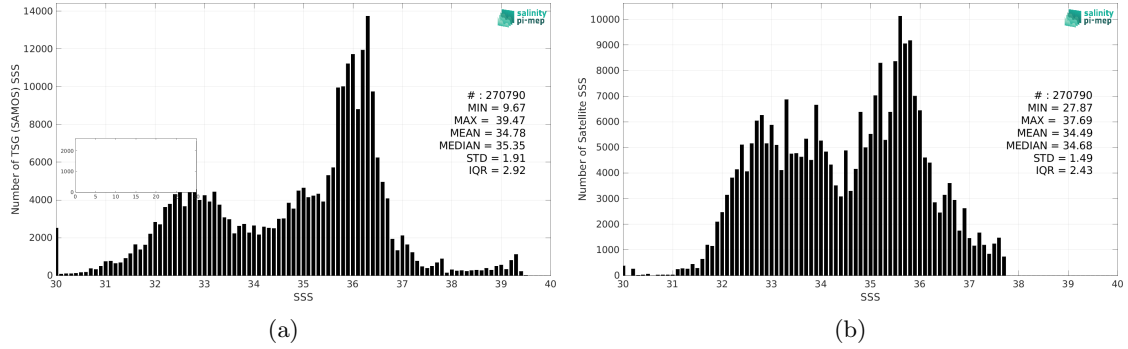
Figure 2: Histograms of SSS from TSG (SAMOS) (a) and Aquarius SSS L4 OI v5 - Weekly (IPRC) (b) considering all match-up pairs per bins of 0.1 over the North Atlantic Ocean Pi-MEP region and for the full satellite product period.
