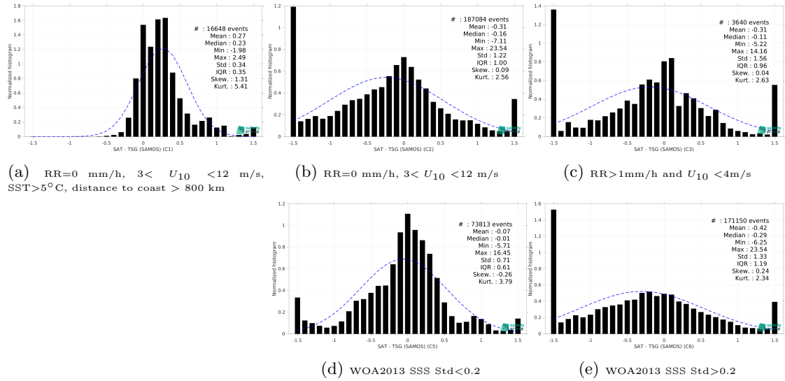
Figure 13: Normalized histogram of \Delta\text{SSS} (Aquarius SSS L4 OI v5 - Weekly (IPRC) - TSG (SAMOS)) for 5 different subdatasets corresponding to: RR=0 mm/h, 3 < U_{10} < 12 m/s, SST>5°C, distance to coast > 800 km (a), RR=0 mm/h, 3 < U_{10} < 12 m/s (b), RR>1mm/h and U_{10} < 4 m/s (c), WOA2013 SSS Std<0.2 (d), WOA2013 SSS Std>0.2 (e).
