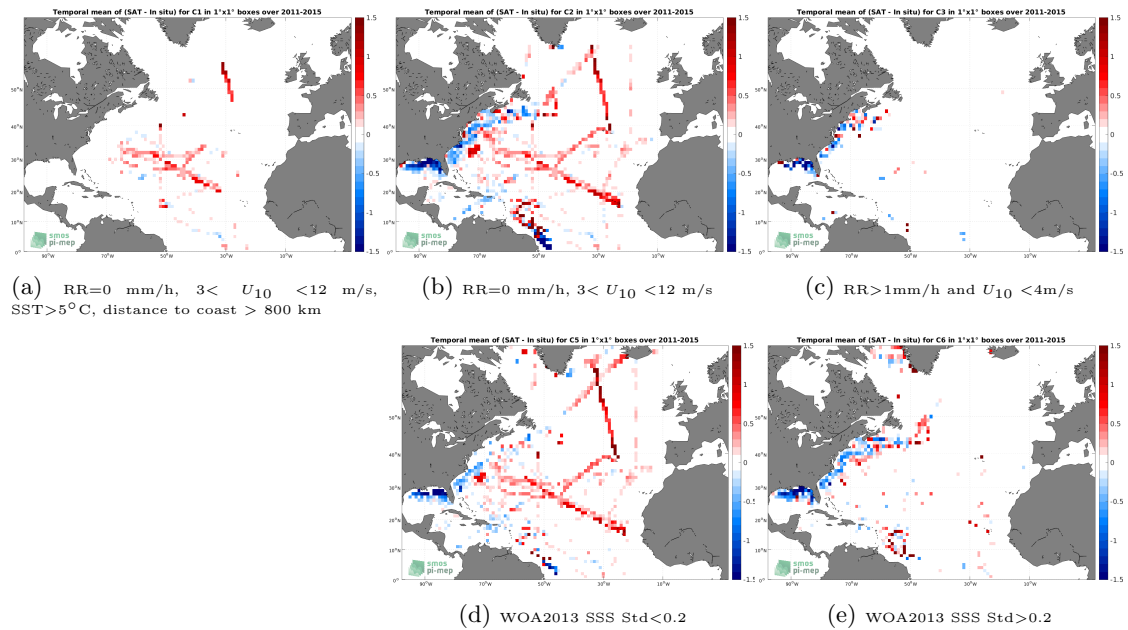
Figure 12: Temporal mean gridded over spatial boxes of size 1^\circ \times 1^\circ of \Delta\text{SSS} (Aquarius SSS L4 OI v5 - Weekly (IPRC) - TSG (SAMOS)) for 5 different subdatasets corresponding to:RR=0 mm/h, 3 < U_{10} < 12 m/s, SST >5^\circ\text{C} , distance to coast > 800 km (a), RR=0 mm/h, 3 < U_{10} < 12 m/s (b), RR >1 mm/h and U_{10} < 4 m/s (c), WOA2013 SSS Std <0.2 (d), WOA2013 SSS Std >0.2 (e).
