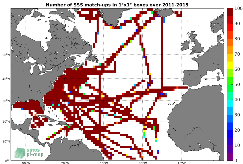
Figure 4: Number of SSS match-ups between TSG-SAMOS SSS and the Aquarius-L4-IPRC-V5-WEEKLY SSS product for the North Atlantic Ocean Pi-MEP region over 1°x1° boxes and for the full satellite product period.
