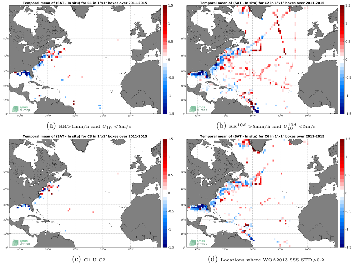
Figure 12: Temporal mean gridded over spatial boxes of size 1^\circ \times 1^\circ of \Delta SSS (Aquarius-L4-IPRC-V5-WEEKLY - TSG-SAMOS) for 4 different subdatasets corresponding to: RR > 1\text{mm/h} and U_{10} < 5\text{m/s} (a), RR^{10d} > 5\text{mm/h} and U_{10}^{10d} < 5\text{m/s} (b), C1 U C2 (c), Locations where WOA2013 SSS STD > 0.2 (d).
