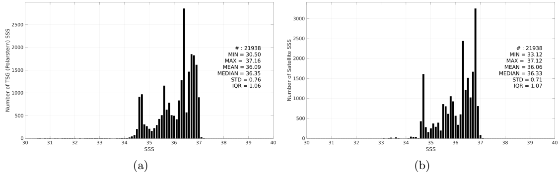
Figure 3: Histograms of SSS from TSG (Polarstern) (a) and Aquarius SSS L4 OI v5 - Weekly (IPRC) (b) considering all match-up pairs per bins of 0.1 over the North Atlantic Ocean Pi-MEP region and for the full satellite product period.
