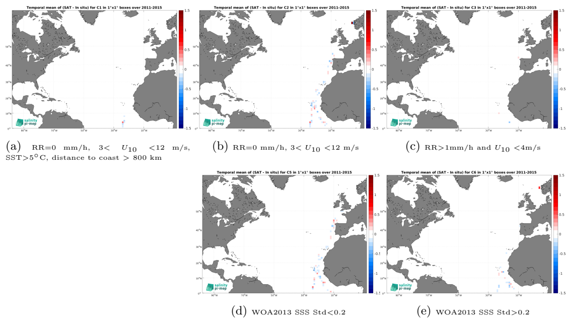
Figure 14: Temporal mean gridded over spatial boxes of size 1^\circ \times 1^\circ of \Delta\text{SSS} (Aquarius SSS L4 OI v5 - Weekly (IPRC) - TSG (Polarstern)) for 5 different subdatasets corresponding to:RR=0 mm/h, 3 < U_{10} < 12 m/s, SST >5^\circ\text{C} , distance to coast > 800 km (a), RR=0 mm/h, 3 < U_{10} < 12 m/s (b), RR >1 mm/h and U_{10} < 4 m/s (c), WOA2013 SSS Std <0.2 (d), WOA2013 SSS Std >0.2 (e).
