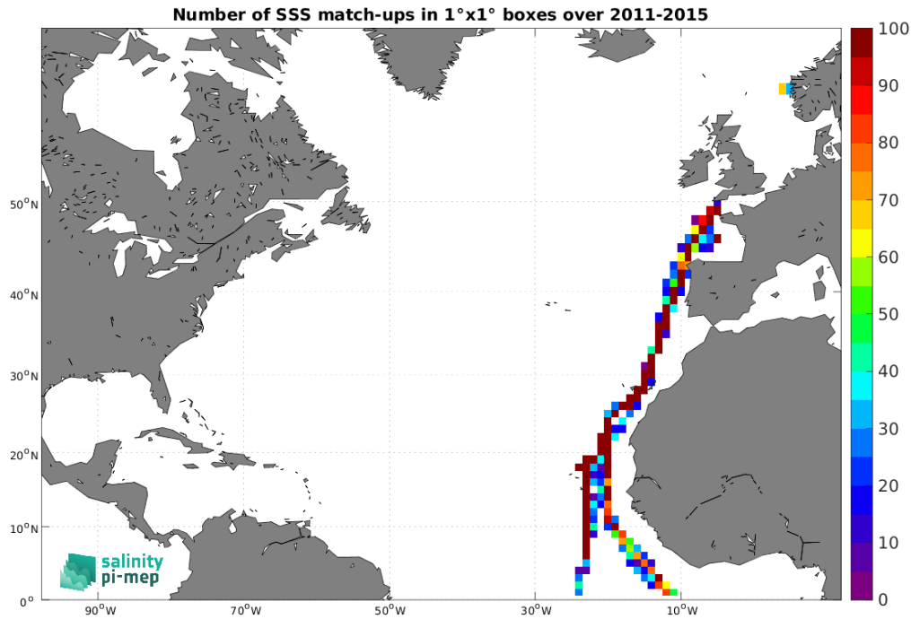
Figure 5: Number of SSS match-ups between TSG (Polarstern) SSS and the Aquarius SSS L4 OI v5 - Weekly (IPRC) SSS product for the North Atlantic Ocean Pi-MEP region over 1^\circ \times 1^\circ boxes and for the full satellite product period.
