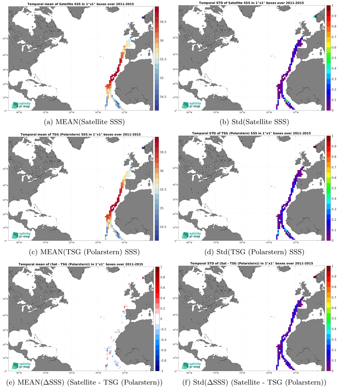
Figure 7: Temporal mean (left) and Std (right) of SSS from Aquarius SSS L4 OI v5 - Weekly (IPRC) (top), TSG (Polarstern) (middle), and of \Delta SSS (Satellite - TSG (Polarstern)). Only match-up pairs are used to generate these maps.
