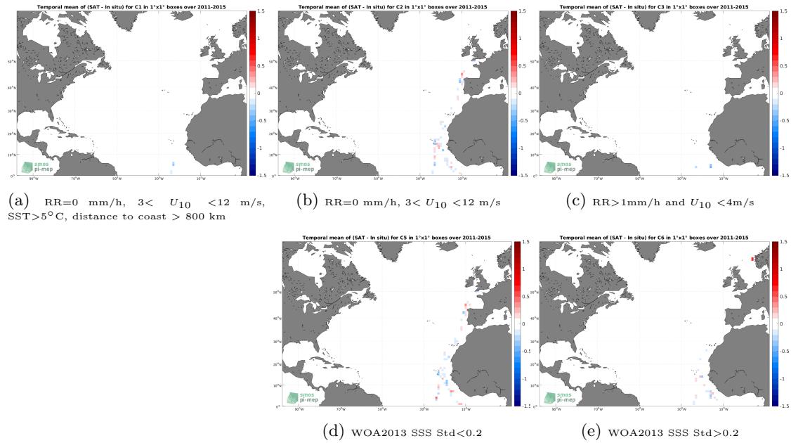
Figure 12: Temporal mean gridded over spatial boxes of size 1^\circ \times 1^\circ of \Delta\text{SSS} (Aquarius SSS L4 OI v5 - Weekly (IPRC) - TSG (Polarstern)) for 5 different subdatasets corresponding to:RR=0 mm/h, 3 < U_{10} < 12 m/s, SST >5^\circ\text{C} , distance to coast > 800 km (a), RR=0 mm/h, 3 < U_{10} < 12 m/s (b), RR >1 mm/h and U_{10} < 4 m/s (c), WOA2013 SSS Std <0.2 (d), WOA2013 SSS Std >0.2 (e).
