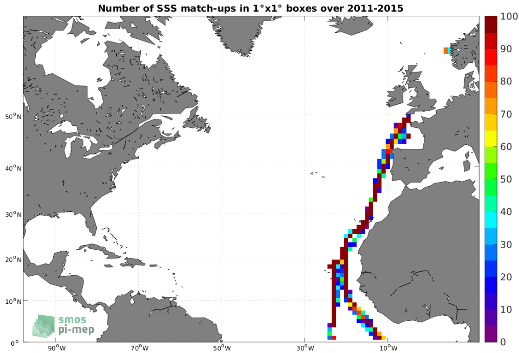
Figure 4: Number of SSS match-ups between TSG (Polarstern) SSS and the Aquarius SSS L4 OI v5 - Weekly (IPRC) SSS product for the North Atlantic Ocean Pi-MEP region over 1^\circ \times 1^\circ boxes and for the full satellite product period.
