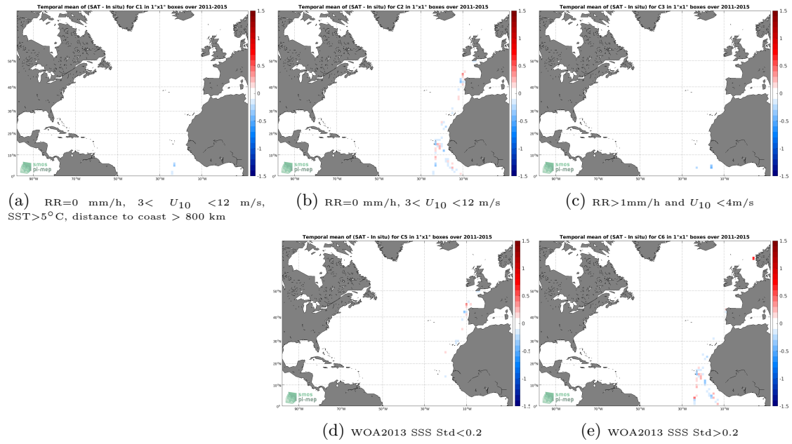
Figure 12: Temporal mean gridded over spatial boxes of size 1^\circ \times 1^\circ of \Delta SSS (Aquarius SSS L4 OI v5 - Weekly (IPRC) - TSG (Polarstern)) for 5 different subdatasets corresponding to:RR=0 mm/h, 3 < U_{10} < 12 m/s, SST>5°C, distance to coast > 800 km (a), RR=0 mm/h, 3 < U_{10} < 12 m/s (b), RR>1mm/h and U_{10} < 4 m/s (c), WOA2013 SSS Std<0.2 (d), WOA2013 SSS Std>0.2 (e).
