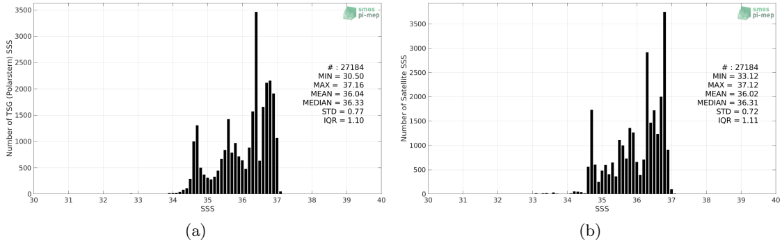
Figure 2: Histograms of SSS from TSG (Polarstern) (a) and Aquarius SSS L4 OI v5 - Weekly (IPRC) (b) considering all match-up pairs per bins of 0.1 over the North Atlantic Ocean Pi-MEP region and for the full satellite product period.
