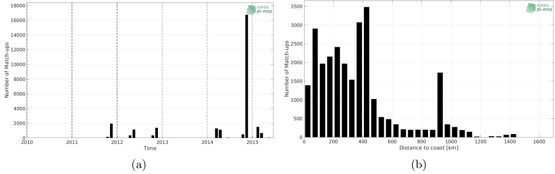
Figure 1: Number of match-ups between TSG (Polarstern) and Aquarius SSS L4 OI v5 - Weekly (IPRC) SSS as a function of time (a) and as function of the distance to coast (b) over the North Atlantic Ocean Pi-MEP region and for the full satellite product period.
