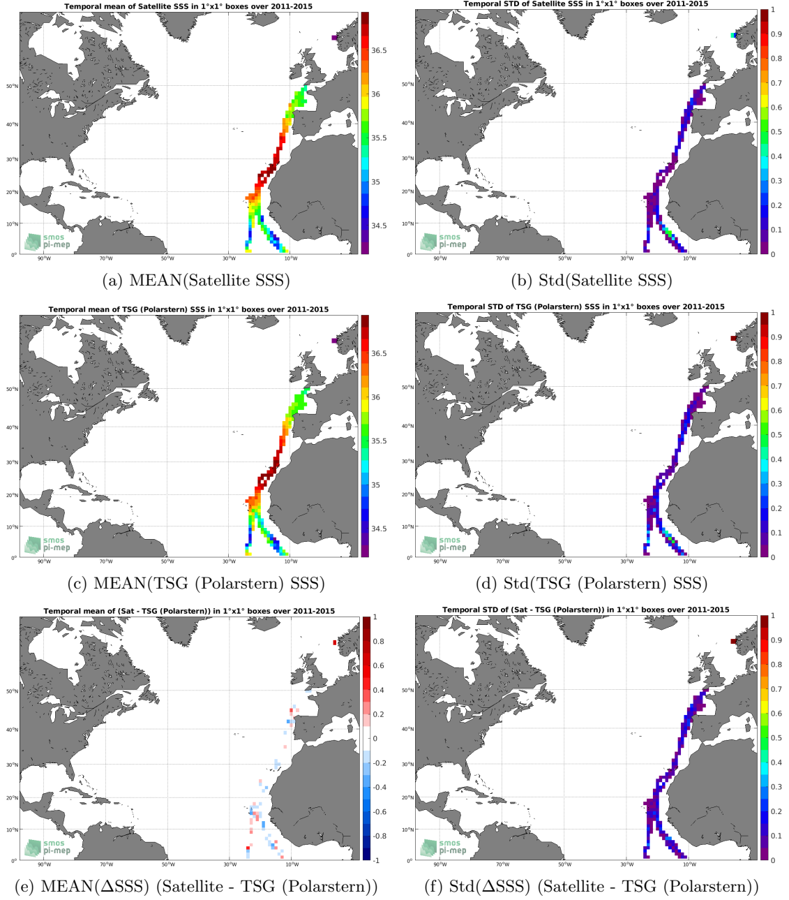
Figure 6: Temporal mean (left) and Std (right) of SSS from Aquarius SSS L4 OI v5 - Weekly (IPRC) (top), TSG (Polarstern) (middle), and of \Delta SSS (Satellite - TSG (Polarstern)). Only match-up pairs are used to generate these maps.
