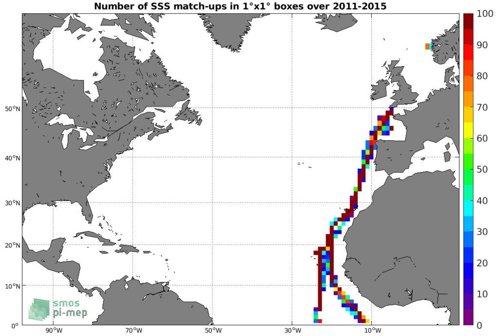
Figure 4: Number of SSS match-ups between TSG (Polarstern) SSS and the Aquarius SSS L4 OI v5 - Weekly (IPRC) SSS product for the North Atlantic Ocean Pi-MEP region over 1°x1° boxes and for the full satellite product period.
