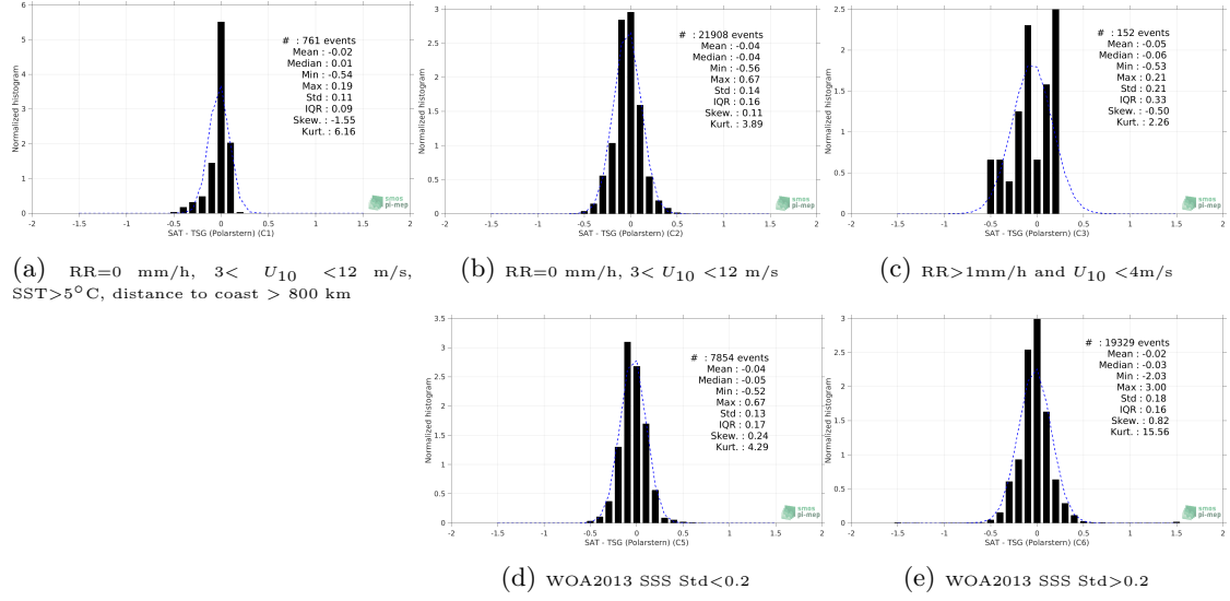
Figure 13: Normalized histogram of \Delta SSS (Aquarius SSS L4 OI v5 - Weekly (IPRC) - TSG (Polarstern)) for 5 different subdatasets corresponding to: RR=0 mm/h, 3 < U_{10} < 12 m/s, SST > 5^\circ C , distance to coast > 800 km (a), RR=0 mm/h, 3 < U_{10} < 12 m/s (b), RR > 1 mm/h and U_{10} < 4 m/s (c), WOA2013 SSS Std < 0.2 (d), WOA2013 SSS Std > 0.2 (e).
