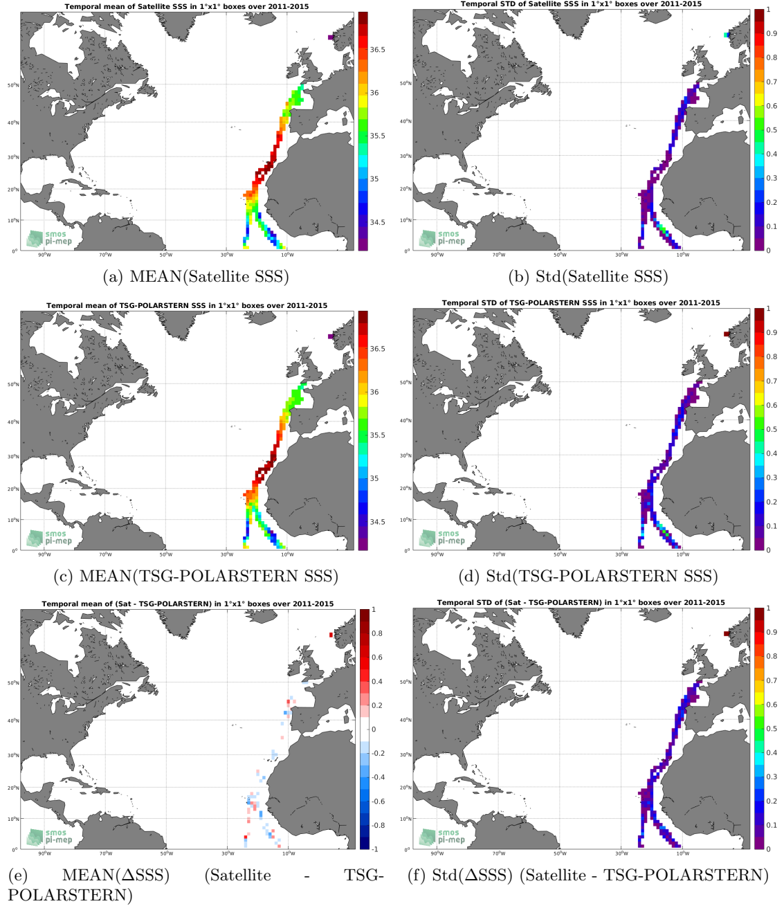
Figure 6: Temporal mean (left) and Std (right) of SSS from Aquarius-L4-IPRC-V5-WEEKLY (top), TSG-POLARSTERN (middle), and of \Delta SSS (Satellite - TSG-POLARSTERN). Only match-up pairs are used to generate these maps.
