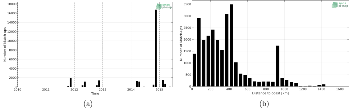
Figure 1: Number of match-ups between TSG-POLARSTERN and Aquarius-L4-IPRC-V5-WEEKLY SSS as a function of time (a) and as function of the distance to coast (b) over the North Atlantic Ocean Pi-MEP region and for the full satellite product period.
