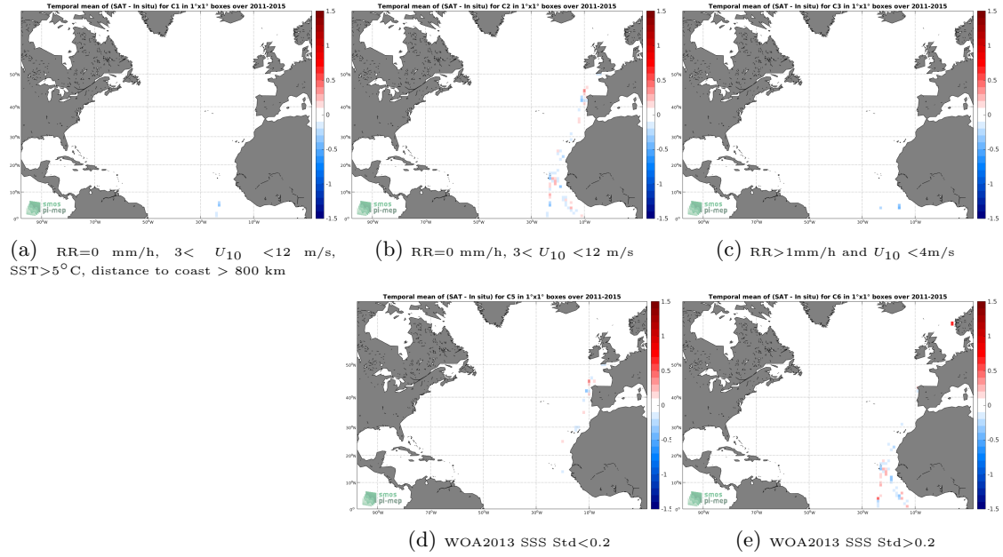
Figure 12: Temporal mean gridded over spatial boxes of size 1^\circ \times 1^\circ of \Delta SSS (Aquarius-L4-IPRC-V5-WEEKLY - TSG-POLARSTERN) for 5 different subdatasets corresponding to:RR=0 mm/h, 3 < U_{10} < 12 m/s, SST >5^\circ\text{C} , distance to coast > 800 km (a), RR=0 mm/h, 3 < U_{10} < 12 m/s (b), RR >1 mm/h and U_{10} < 4 m/s (c), WOA2013 SSS Std <0.2 (d), WOA2013 SSS Std >0.2 (e).
