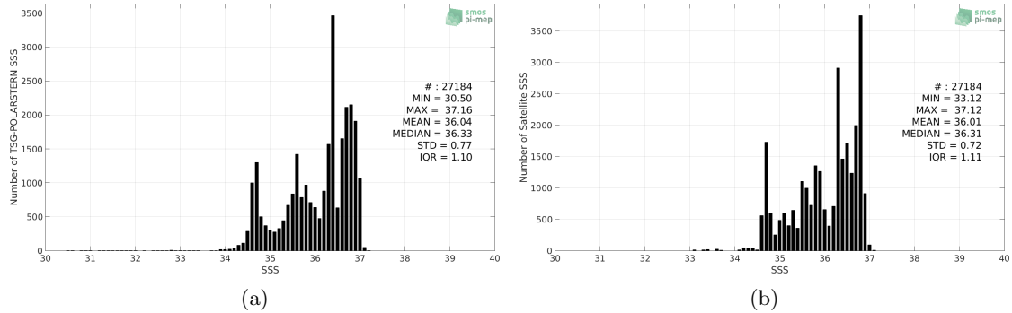
Figure 2: Histograms of SSS from TSG-POLARSTERN (a) and Aquarius-L4-IPRC-V5-WEEKLY (b) considering all match-up pairs per bins of 0.1 over the North Atlantic Ocean Pi-MEP region and for the full satellite product period.
