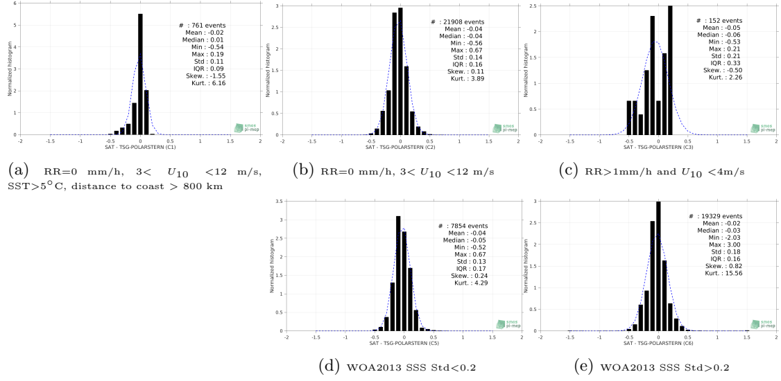
Figure 13: Normalized histogram of \Delta SSS (Aquarius-L4-IPRC-V5-WEEKLY - TSG-POLARSTERN) for 5 different subdatasets corresponding to: RR=0 mm/h, 3 < U_{10} < 12 m/s, SST>5°C, distance to coast > 800 km (a), RR=0 mm/h, 3 < U_{10} < 12 m/s (b), RR>1 mm/h and U_{10} < 4 m/s (c), WOA2013 SSS Std<0.2 (d), WOA2013 SSS Std>0.2 (e).
