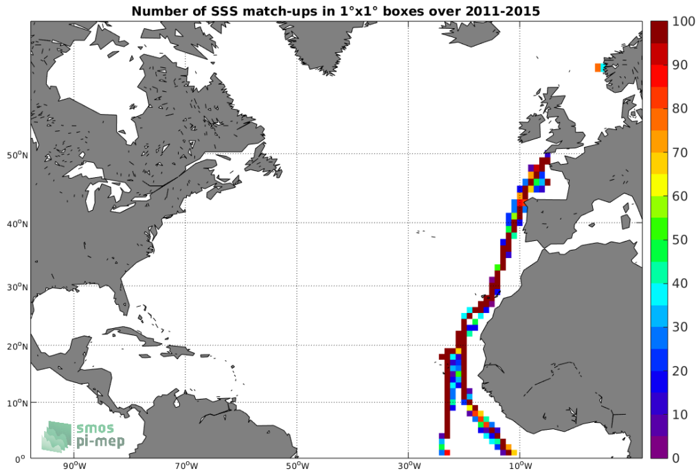
Figure 4: Number of SSS match-ups between TSG-POLARSTERN SSS and the Aquarius-L4-IPRC-V5-WEEKLY SSS product for the North Atlantic Ocean Pi-MEP region over 1^\circ \times 1^\circ boxes and for the full satellite product period.
