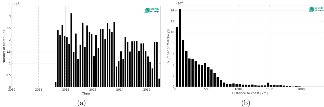
Figure 2: Number of match-ups between TSG (LEGOS-DM) and Aquarius SSS L4 OI v5 - Weekly (IPRC) SSS as a function of time (a) and as function of the distance to coast (b) over the North Atlantic Ocean Pi-MEP region and for the full satellite product period.
