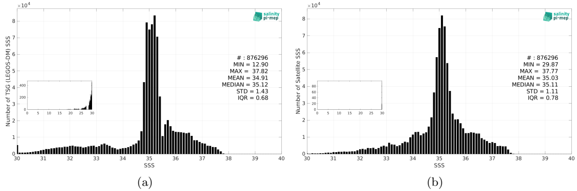
Figure 3: Histograms of SSS from TSG (LEGOS-DM) (a) and Aquarius SSS L4 OI v5 - Weekly (IPRC) (b) considering all match-up pairs per bins of 0.1 over the North Atlantic Ocean Pi-MEP region and for the full satellite product period.
