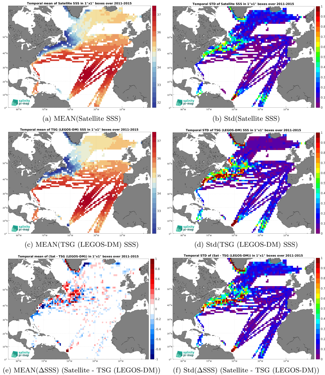
Figure 7: Temporal mean (left) and Std (right) of SSS from Aquarius SSS L4 OI v5 - Weekly (IPRC) (top), TSG (LEGOS-DM) (middle), and of \Delta SSS (Satellite - TSG (LEGOS-DM)). Only match-up pairs are used to generate these maps.
