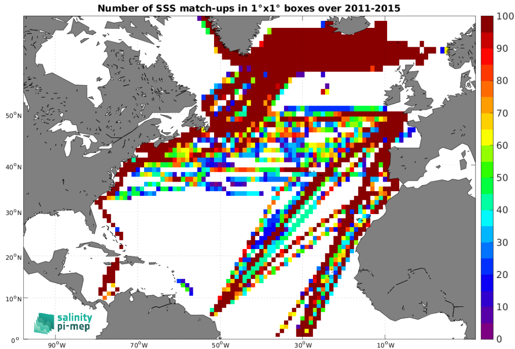
Figure 5: Number of SSS match-ups between TSG (LEGOS-DM) SSS and the Aquarius SSS L4 OI v5 - Weekly (IPRC) SSS product for the North Atlantic Ocean Pi-MEP region over 1^\circ \times 1^\circ boxes and for the full satellite product period.
