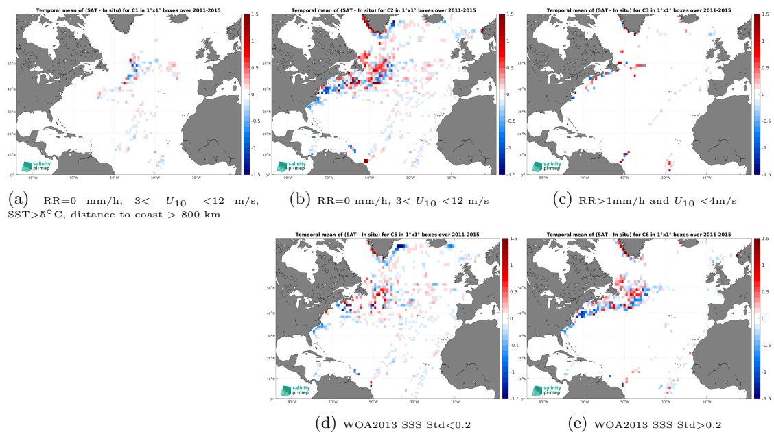
Figure 14: Temporal mean gridded over spatial boxes of size 1^\circ \times 1^\circ of \Delta\text{SSS} (Aquarius SSS L4 OI v5 - Weekly (IPRC) - TSG (LEGOS-DM)) for 5 different subdatasets corresponding to:RR=0 mm/h, 3 < U_{10} < 12 m/s, SST >5^\circ\text{C} , distance to coast > 800 km (a), RR=0 mm/h, 3 < U_{10} < 12 m/s (b), RR >1 mm/h and U_{10} < 4 m/s (c), WOA2013 SSS Std <0.2 (d), WOA2013 SSS Std >0.2 (e).
