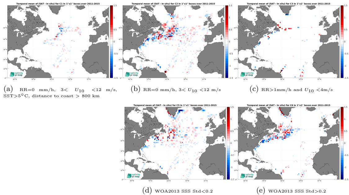
Figure 12: Temporal mean gridded over spatial boxes of size 1^\circ \times 1^\circ of \Delta\text{SSS} (Aquarius SSS L4 OI v5 - Weekly (IPRC) - TSG (LEGOS-DM)) for 5 different subdatasets corresponding to:RR=0 mm/h, 3 < U_{10} < 12 m/s, SST >5^\circ\text{C} , distance to coast > 800 km (a), RR=0 mm/h, 3 < U_{10} < 12 m/s (b), RR >1 mm/h and U_{10} < 4 m/s (c), WOA2013 SSS Std <0.2 (d), WOA2013 SSS Std >0.2 (e).
