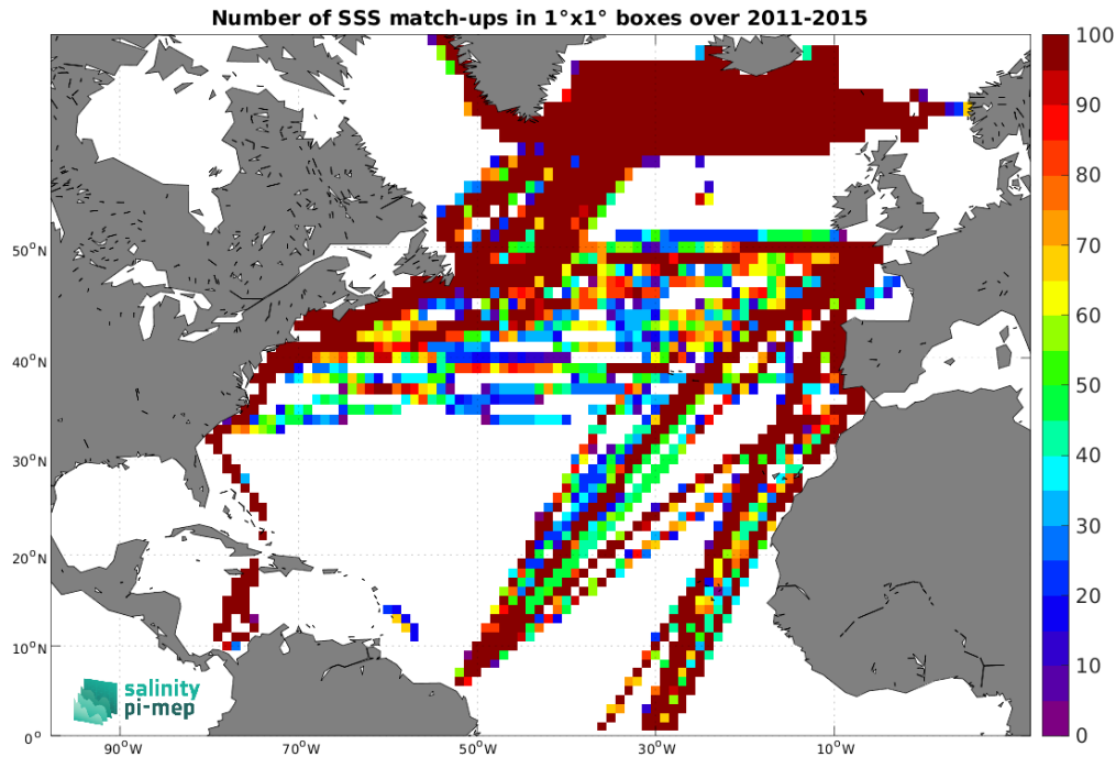
Figure 4: Number of SSS match-ups between TSG (LEGOS-DM) SSS and the Aquarius SSS L4 OI v5 - Weekly (IPRC) SSS product for the North Atlantic Ocean Pi-MEP region over 1^\circ \times 1^\circ boxes and for the full satellite product period.
