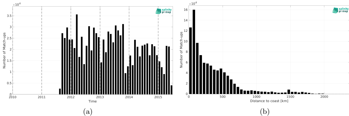
Figure 1: Number of match-ups between TSG (LEGOS-DM) and Aquarius SSS L4 OI v5 - Weekly (IPRC) SSS as a function of time (a) and as function of the distance to coast (b) over the North Atlantic Ocean Pi-MEP region and for the full satellite product period.
