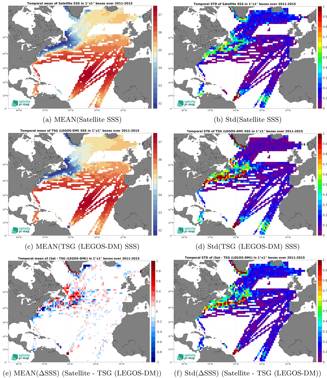
Figure 6: Temporal mean (left) and Std (right) of SSS from Aquarius SSS L4 OI v5 - Weekly (IPRC) (top), TSG (LEGOS-DM) (middle), and of \Delta SSS (Satellite - TSG (LEGOS-DM)). Only match-up pairs are used to generate these maps.
