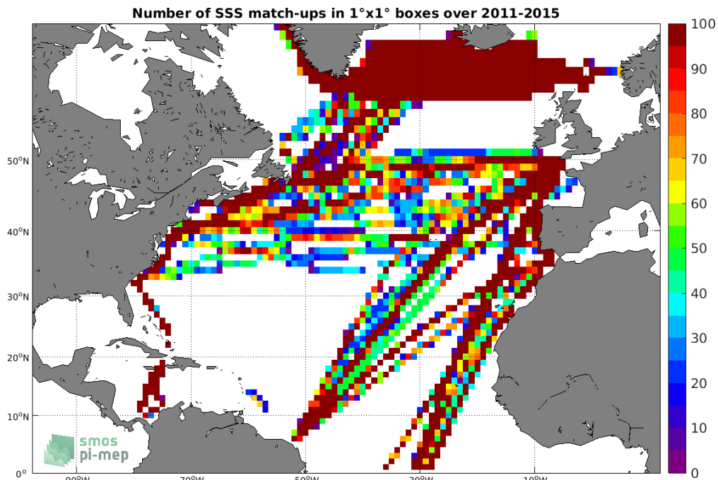
Figure 4: Number of SSS match-ups between TSG (LEGOS-DM) SSS and the Aquarius SSS L4 OI v5 - Weekly (IPRC) SSS product for the North Atlantic Ocean Pi-MEP region over 1°x1° boxes and for the full satellite product period.
