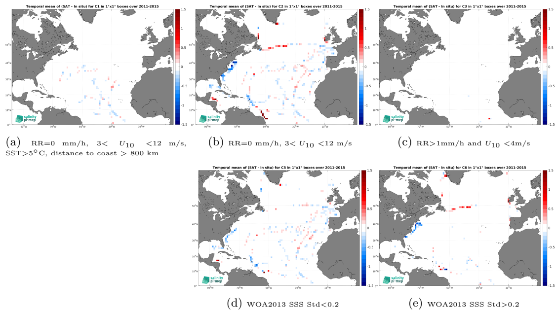
Figure 12: Temporal mean gridded over spatial boxes of size 1^\circ \times 1^\circ of \Delta\text{SSS} (Aquarius SSS L4 OI v5 - Weekly (IPRC) - TSG (GOSUD-Sailing-ship)) for 5 different subdatasets corresponding to:RR=0 mm/h, 3 < U_{10} < 12 m/s, SST >5^\circ\text{C} , distance to coast > 800 km (a), RR=0 mm/h, 3 < U_{10} < 12 m/s (b), RR >1 mm/h and U_{10} < 4 m/s (c), WOA2013 SSS Std <0.2 (d), WOA2013 SSS Std >0.2 (e).
