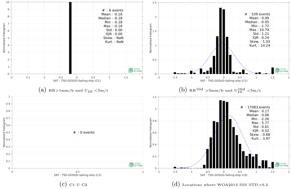
Figure 13: Normalized histogram of \Delta SSS (Aquarius-L4-IPRC-V5-WEEKLY - TSG-GOSUD-Sailing-ship) for 6 different subdatasets corresponding to: RR > 1mm/h and U_{10} < 5 m/s (a), RR^{10d} > 5 mm/h and U_{10}^{10d} < 5 m/s (b), C1 U C2 (c), Locations where WOA2013 SSS STD > 0.2 (d).
