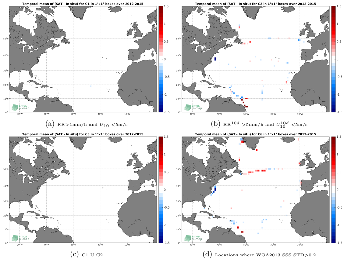
Figure 12: Temporal mean gridded over spatial boxes of size 1^\circ \times 1^\circ of \Delta SSS (Aquarius-L4-IPRC-V5-WEEKLY - TSG-GOSUD-Sailing-ship) for 4 different subdatasets corresponding to: RR > 1mm/h and U_{10} < 5\text{m/s} (a), RR^{10d} > 5\text{mm/h} and U_{10}^{10d} < 5\text{m/s} (b), C1 U C2 (c), Locations where WOA2013 SSS STD > 0.2 (d).
