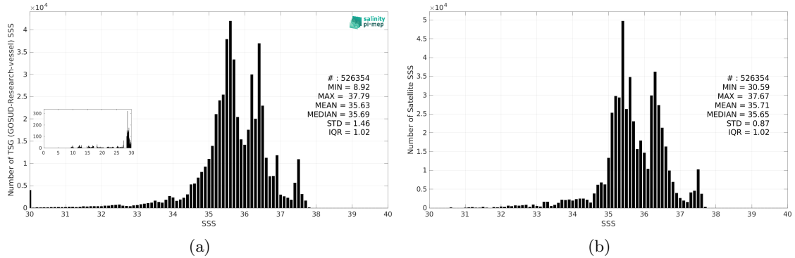
Figure 3: Histograms of SSS from TSG (GOSUD-Research-vessel) (a) and Aquarius SSS L4 OI v5 - Weekly (IPRC) (b) considering all match-up pairs per bins of 0.1 over the North Atlantic Ocean Pi-MEP region and for the full satellite product period.
