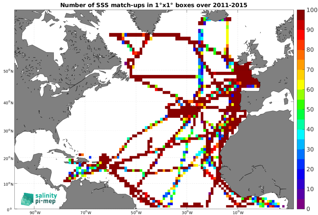
Figure 5: Number of SSS match-ups between TSG (GOSUD-Research-vessel) SSS and the Aquarius SSS L4 OI v5 - Weekly (IPRC) SSS product for the North Atlantic Ocean Pi-MEP region over 1^\circ \times 1^\circ boxes and for the full satellite product period.
