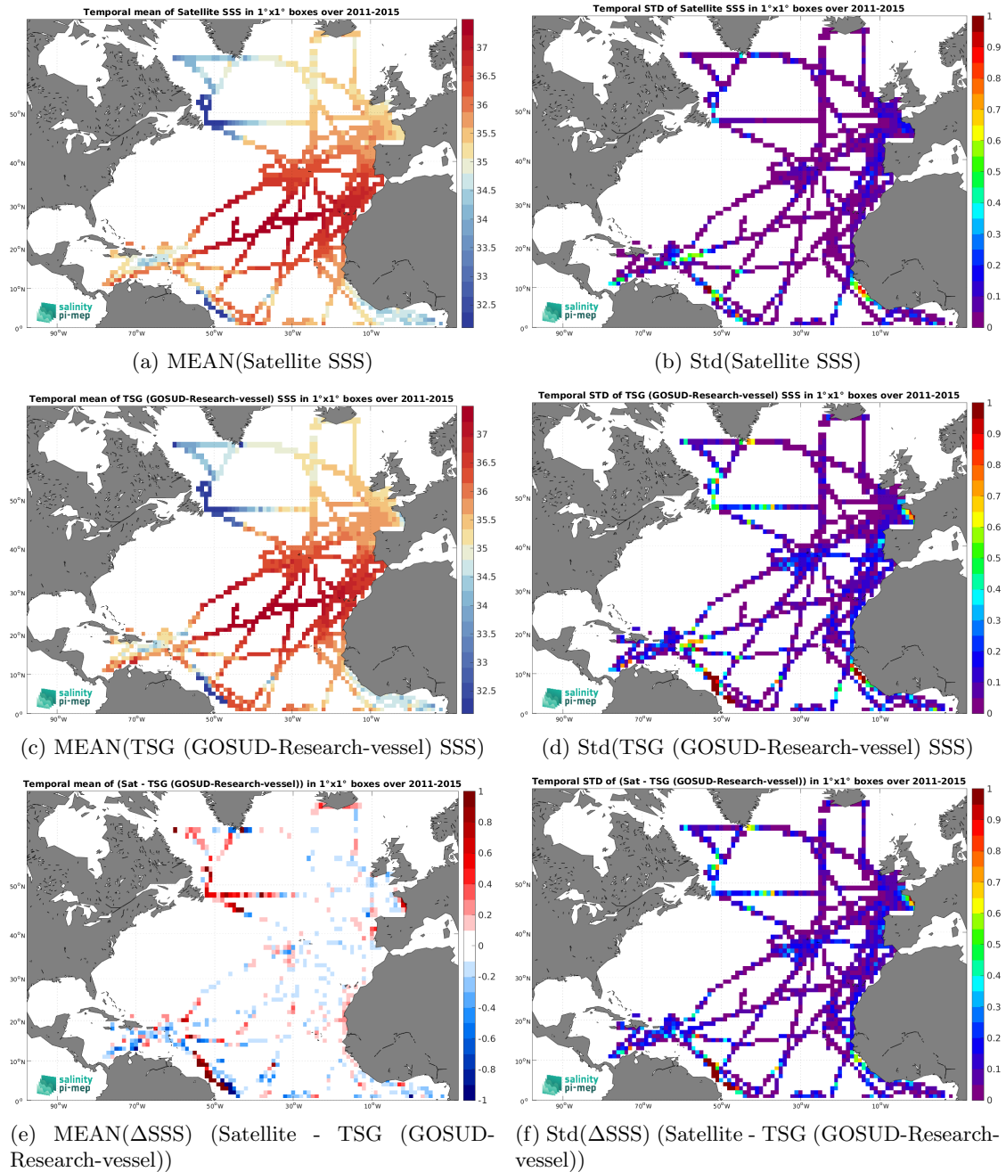
Figure 7: Temporal mean (left) and Std (right) of SSS from Aquarius SSS L4 OI v5 - Weekly (IPRC) (top), TSG (GOSUD-Research-vessel) (middle), and of \Delta SSS (Satellite - TSG (GOSUD-Research-vessel)). Only match-up pairs are used to generate these maps.
