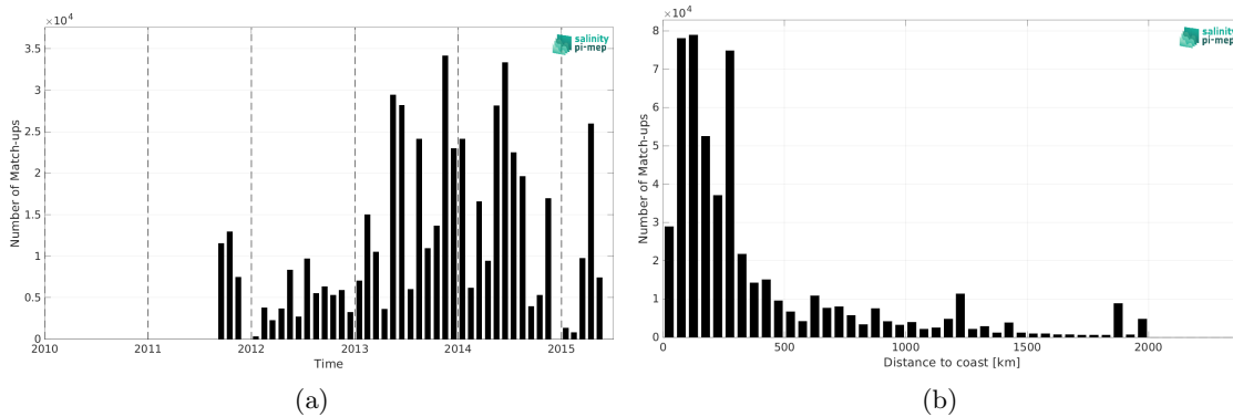
Figure 2: Number of match-ups between TSG (GOSUD-Research-vessel) and Aquarius SSS L4 OI v5 - Weekly (IPRC) SSS as a function of time (a) and as function of the distance to coast (b) over the North Atlantic Ocean Pi-MEP region and for the full satellite product period.
