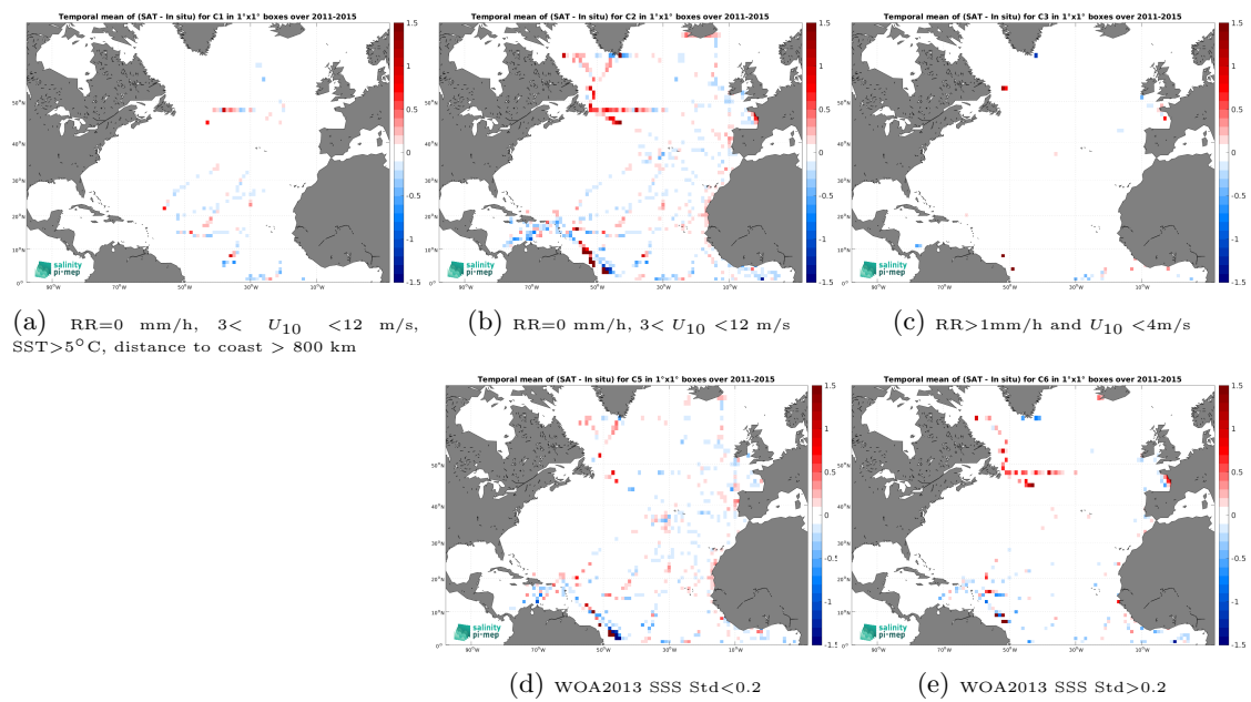
Figure 14: Temporal mean gridded over spatial boxes of size 1^\circ \times 1^\circ of \Delta\text{SSS} (Aquarius SSS L4 OI v5 - Weekly (IPRC) - TSG (GOSUD-Research-vessel)) for 5 different subdatasets corresponding to:RR=0 mm/h, 3 < U_{10} < 12 m/s, SST >5^\circ\text{C} , distance to coast > 800 km (a), RR=0 mm/h, 3 < U_{10} < 12 m/s (b), RR >1 mm/h and U_{10} < 4 m/s (c), WOA2013 SSS Std <0.2 (d), WOA2013 SSS Std >0.2 (e).
