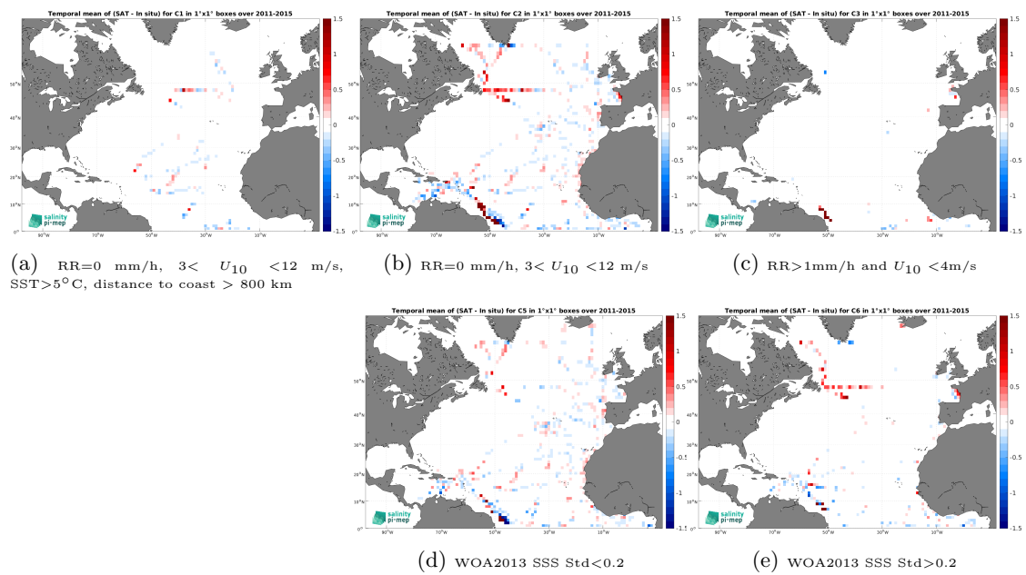
Figure 12: Temporal mean gridded over spatial boxes of size 1^\circ \times 1^\circ of \Delta\text{SSS} (Aquarius SSS L4 OI v5 - Weekly (IPRC) - TSG (GOSUD-Research-vessel)) for 5 different subdatasets corresponding to:RR=0 mm/h, 3 < U_{10} < 12 m/s, SST >5^\circ\text{C} , distance to coast > 800 km (a), RR=0 mm/h, 3 < U_{10} < 12 m/s (b), RR >1 mm/h and U_{10} < 4 m/s (c), WOA2013 SSS Std <0.2 (d), WOA2013 SSS Std >0.2 (e).
