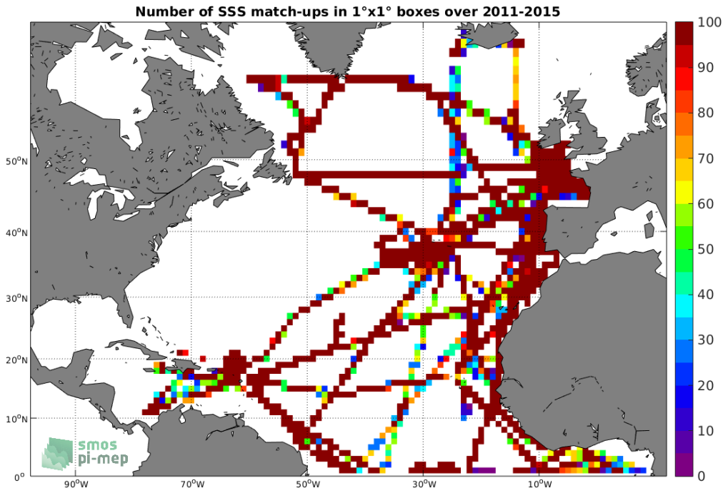
Figure 4: Number of SSS match-ups between TSG-GOSUD-Research-vessel SSS and the Aquarius-L4-IPRC-V5-WEEKLY SSS product for the North Atlantic Ocean Pi-MEP region over 1°x1° boxes and for the full satellite product period.
