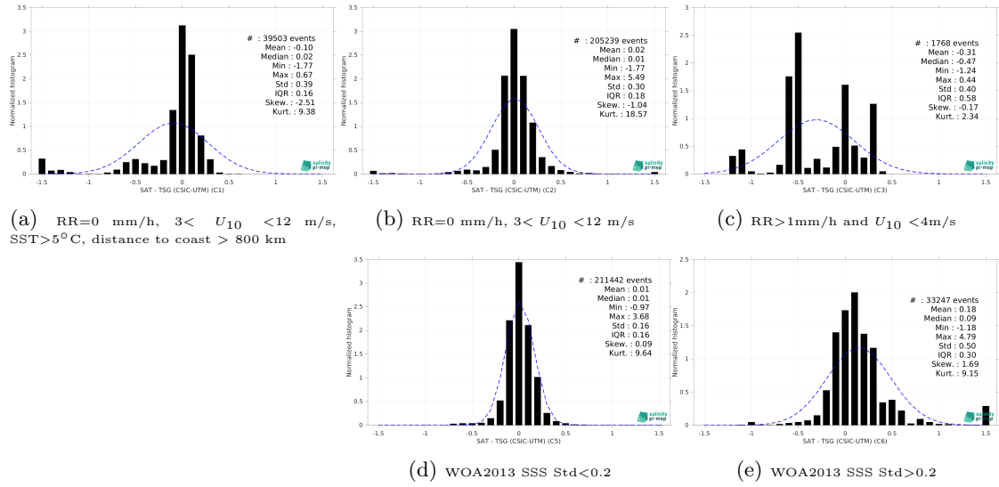
Figure 15: Normalized histogram of \Delta\text{SSS} (Aquarius SSS L4 OI v5 - Weekly (IPRC) - TSG (CSIC-UTM)) for 5 different subdatasets corresponding to: RR=0 mm/h, 3 < U_{10} < 12 m/s, SST > 5^\circ\text{C} , distance to coast > 800 km (a), RR=0 mm/h, 3 < U_{10} < 12 m/s (b), RR > 1 mm/h and U_{10} < 4 m/s (c), WOA2013 SSS Std < 0.2 (d), WOA2013 SSS Std > 0.2 (e).
