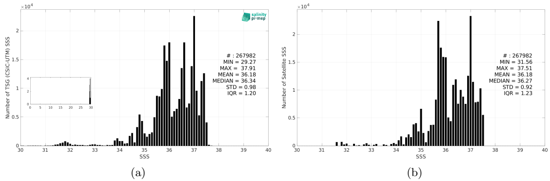
Figure 3: Histograms of SSS from TSG (CSIC-UTM) (a) and Aquarius SSS L4 OI v5 - Weekly (IPRC) (b) considering all match-up pairs per bins of 0.1 over the North Atlantic Ocean Pi-MEP region and for the full satellite product period.
