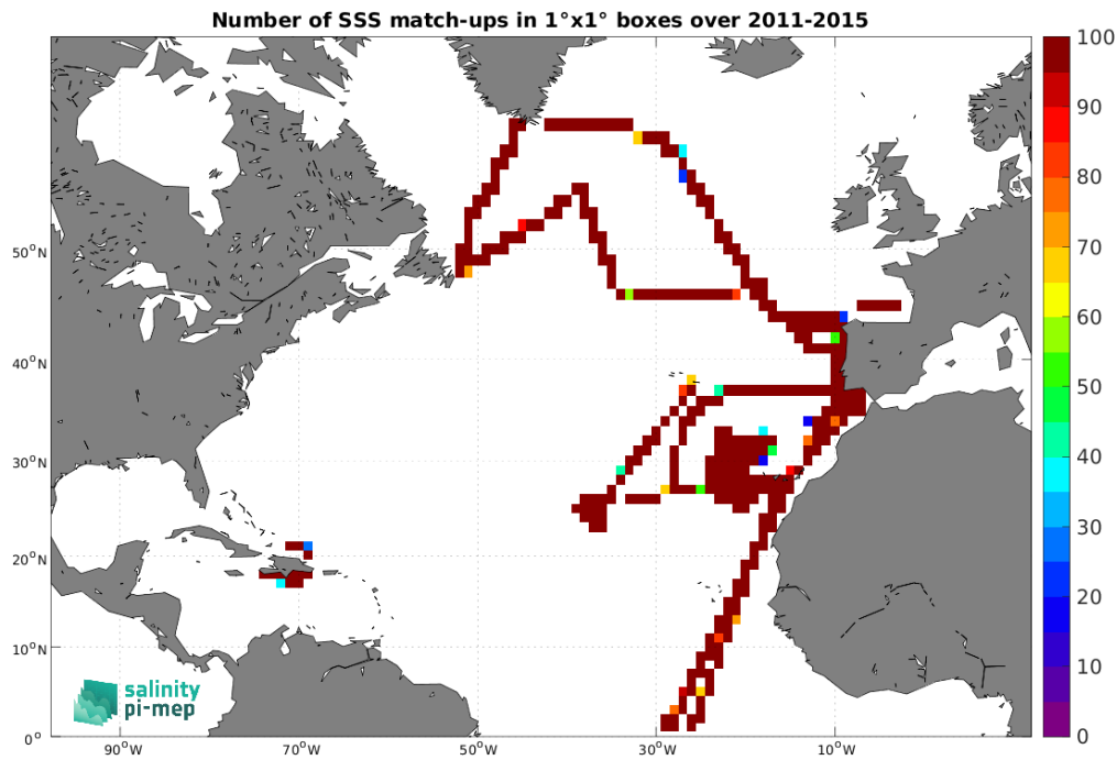
Figure 5: Number of SSS match-ups between TSG (CSIC-UTM) SSS and the Aquarius SSS L4 OI v5 - Weekly (IPRC) SSS product for the North Atlantic Ocean Pi-MEP region over 1^\circ \times 1^\circ boxes and for the full satellite product period.
