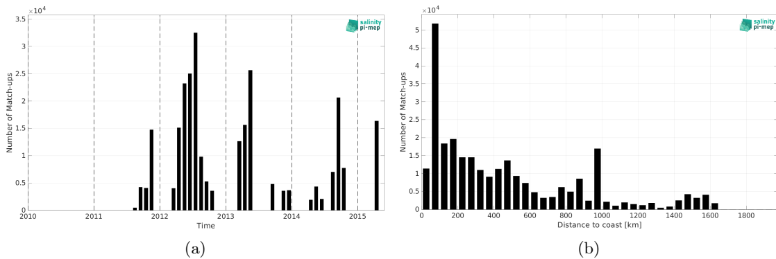
Figure 2: Number of match-ups between TSG (CSIC-UTM) and Aquarius SSS L4 OI v5 - Weekly (IPRC) SSS as a function of time (a) and as function of the distance to coast (b) over the North Atlantic Ocean Pi-MEP region and for the full satellite product period.
