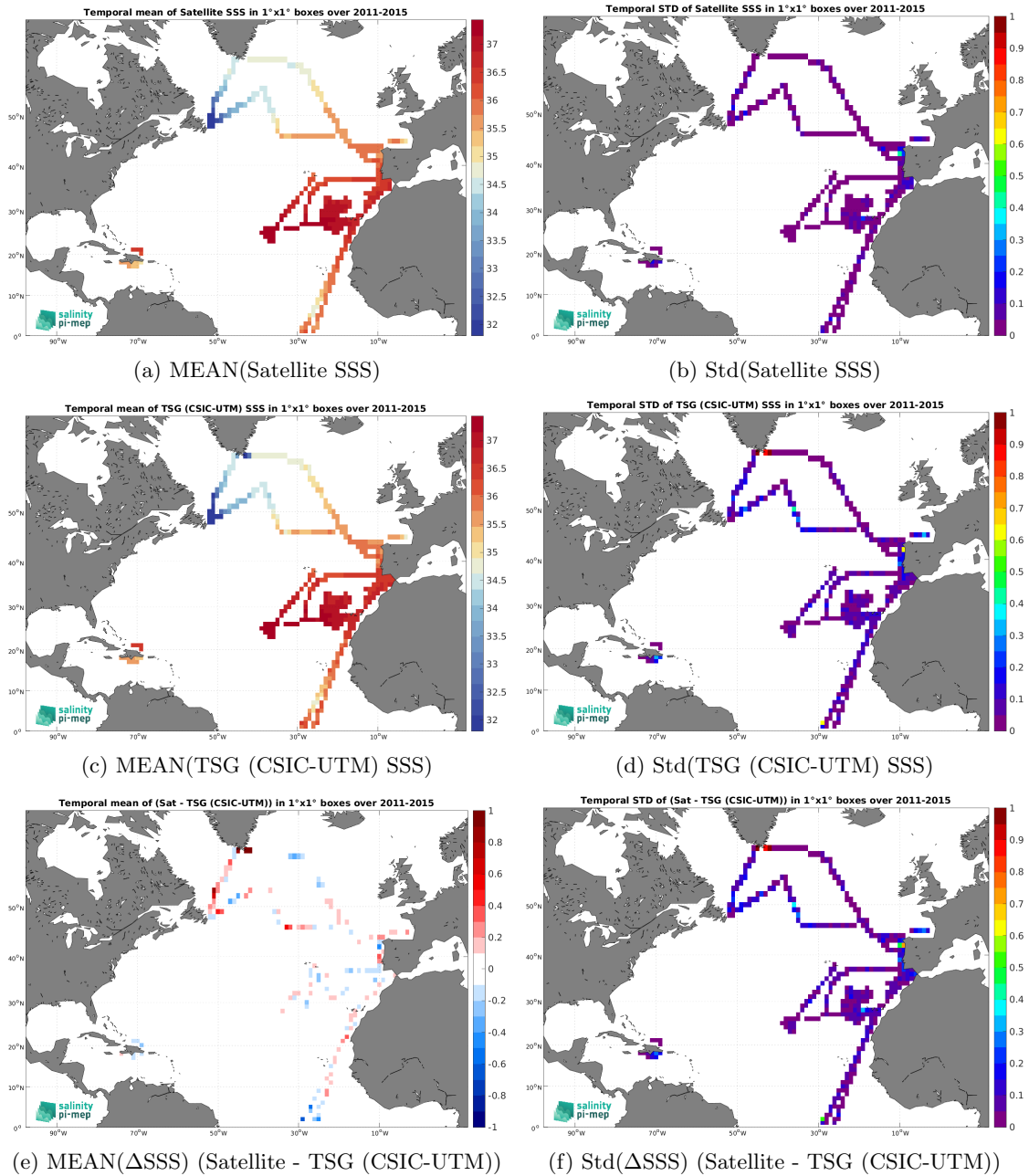
Figure 7: Temporal mean (left) and Std (right) of SSS from Aquarius SSS L4 OI v5 - Weekly (IPRC) (top), TSG (CSIC-UTM) (middle), and of \Delta SSS (Satellite - TSG (CSIC-UTM)). Only match-up pairs are used to generate these maps.
