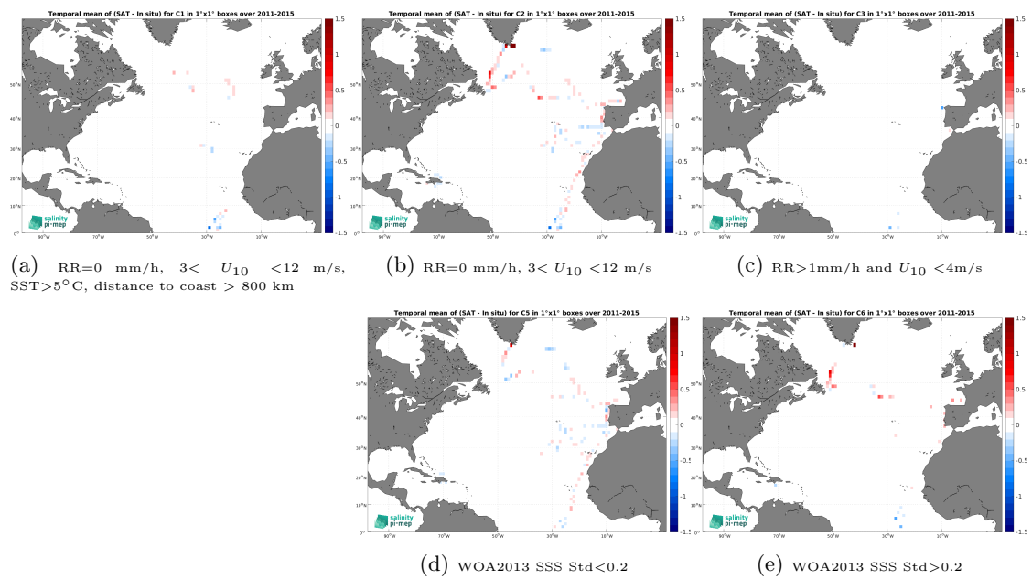
Figure 14: Temporal mean gridded over spatial boxes of size 1^\circ \times 1^\circ of \Delta\text{SSS} (Aquarius SSS L4 OI v5 - Weekly (IPRC) - TSG (CSIC-UTM)) for 5 different subdatasets corresponding to:RR=0 mm/h, 3 < U_{10} < 12 m/s, SST > 5°C, distance to coast > 800 km (a), RR=0 mm/h, 3 < U_{10} < 12 m/s (b), RR > 1mm/h and U_{10} < 4 m/s (c), WOA2013 SSS Std < 0.2 (d), WOA2013 SSS Std > 0.2 (e).
