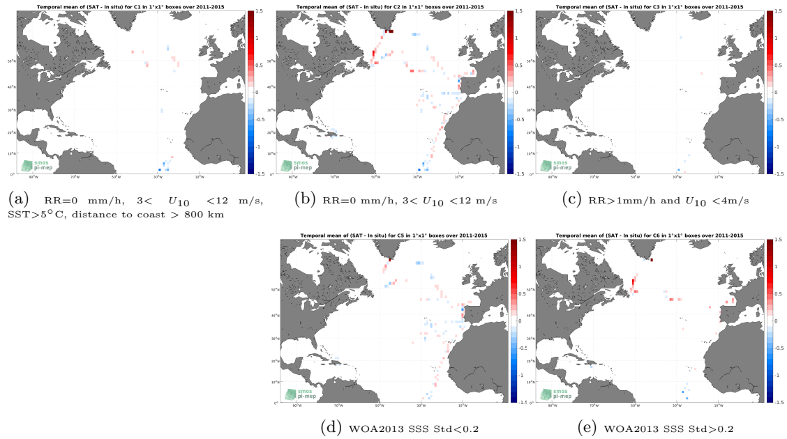
Figure 12: Temporal mean gridded over spatial boxes of size 1^\circ \times 1^\circ of \Delta SSS (Aquarius SSS L4 OI v5 - Weekly (IPRC) - TSG (CSIC-UTM)) for 5 different subdatasets corresponding to:RR=0 mm/h, 3 < U_{10} < 12 m/s, SST >5^\circ C, distance to coast > 800 km (a), RR=0 mm/h, 3 < U_{10} < 12 m/s (b), RR >1 mm/h and U_{10} < 4 m/s (c), WOA2013 SSS Std <0.2 (d), WOA2013 SSS Std >0.2 (e).
