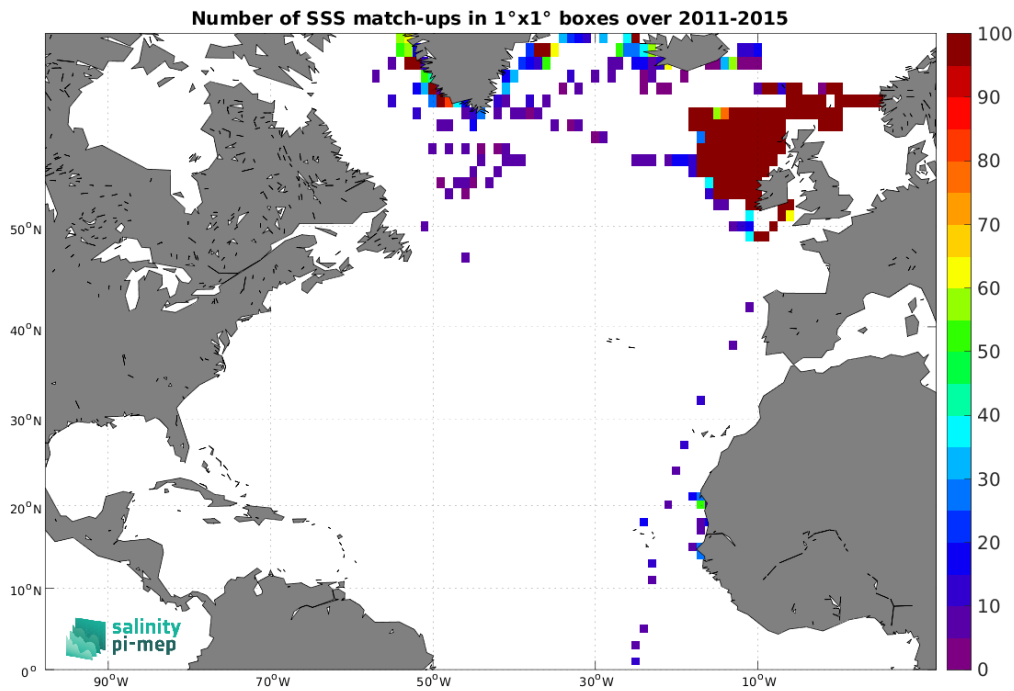
Figure 5: Number of SSS match-ups between ICES SSS and the Aquarius SSS L4 OI v5 - Weekly (IPRC) SSS product for the North Atlantic Ocean Pi-MEP region over 1^{\circ} \times 1^{\circ} boxes and for the full satellite product period.
