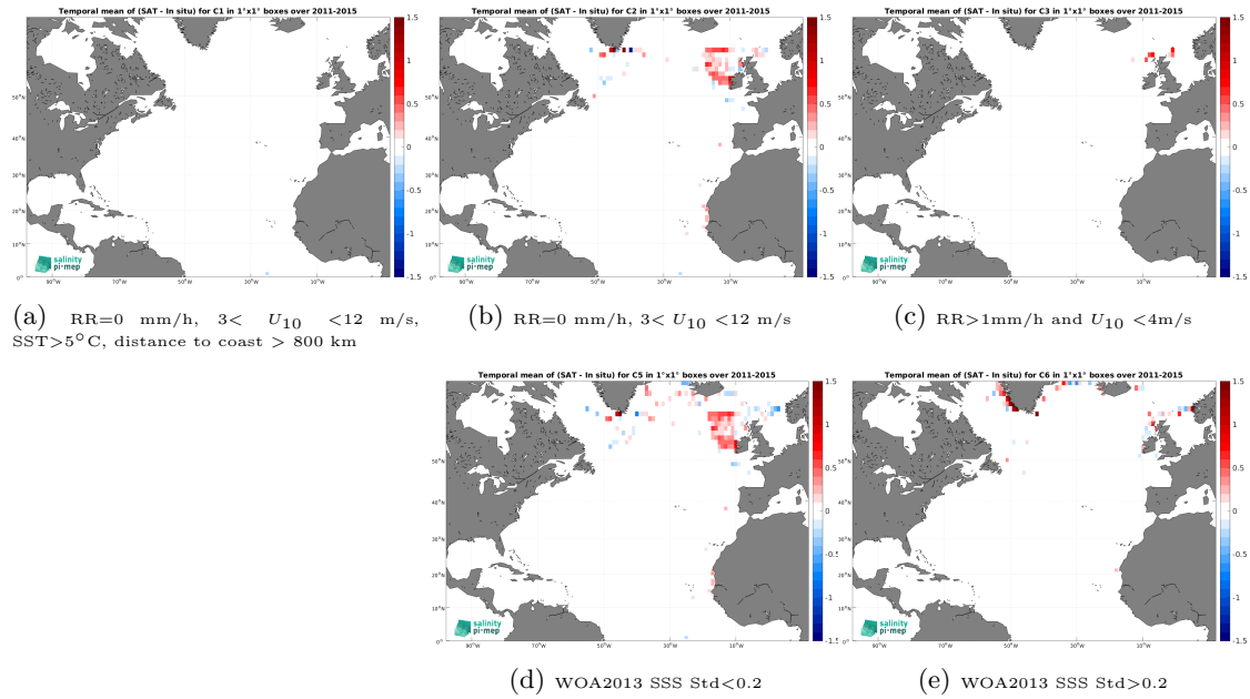
Figure 12: Temporal mean gridded over spatial boxes of size 1^\circ \times 1^\circ of \Delta\text{SSS} (Aquarius SSS L4 OI v5 - Weekly (IPRC) - ICES) for 5 different subdatasets corresponding to:RR=0 mm/h, 3 < U_{10} < 12 m/s, SST >5^\circ\text{C} , distance to coast > 800 km (a), RR=0 mm/h, 3 < U_{10} < 12 m/s (b), RR >1 mm/h and U_{10} < 4 m/s (c), WOA2013 SSS Std <0.2 (d), WOA2013 SSS Std >0.2 (e).
