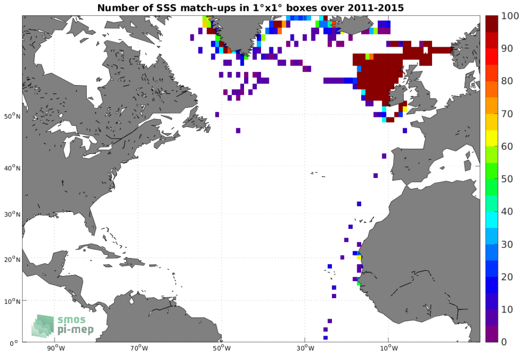
Figure 4: Number of SSS match-ups between ICES SSS and the Aquarius SSS L4 OI v5 - Weekly (IPRC) SSS product for the North Atlantic Ocean Pi-MEP region over 1^{\circ} \times 1^{\circ} boxes and for the full satellite product period.
