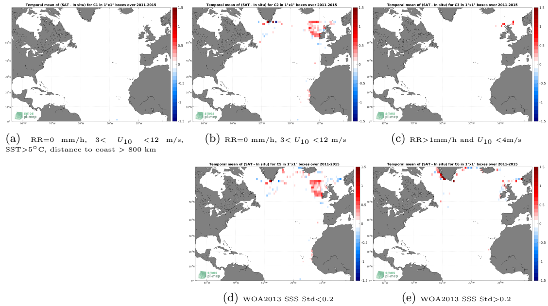
Figure 12: Temporal mean gridded over spatial boxes of size 1^\circ \times 1^\circ of \Delta SSS (Aquarius SSS L4 OI v5 - Weekly (IPRC) - ICES) for 5 different subdatasets corresponding to:RR=0 mm/h, 3 < U_{10} < 12 m/s, SST >5^\circ\text{C} , distance to coast > 800 km (a), RR=0 mm/h, 3 < U_{10} < 12 m/s (b), RR >1 mm/h and U_{10} < 4 m/s (c), WOA2013 SSS Std <0.2 (d), WOA2013 SSS Std >0.2 (e).
