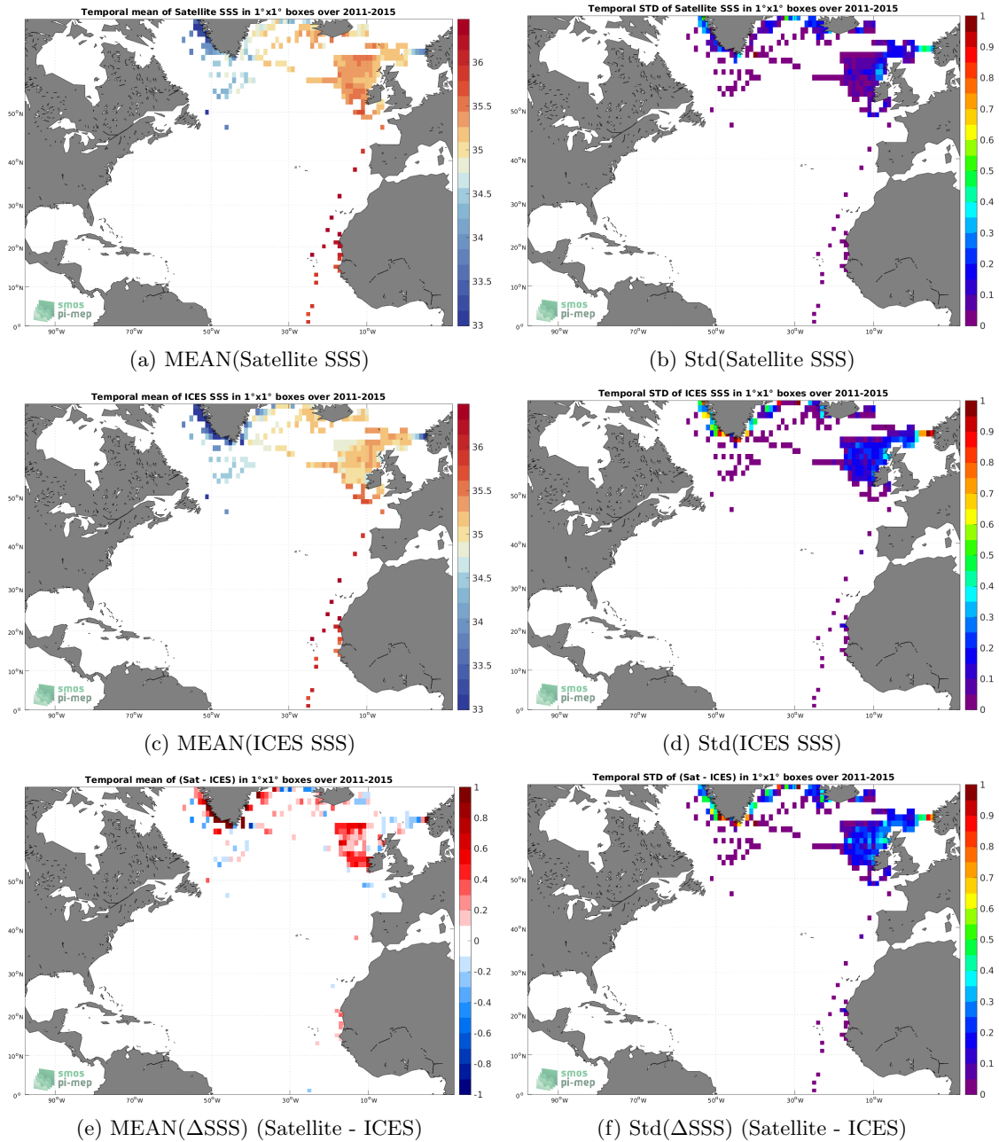
Figure 6: Temporal mean (left) and Std (right) of SSS from Aquarius SSS L4 OI v5 - Weekly (IPRC) (top), ICES (middle), and of \Delta SSS (Satellite - ICES). Only match-up pairs are used to generate these maps.
