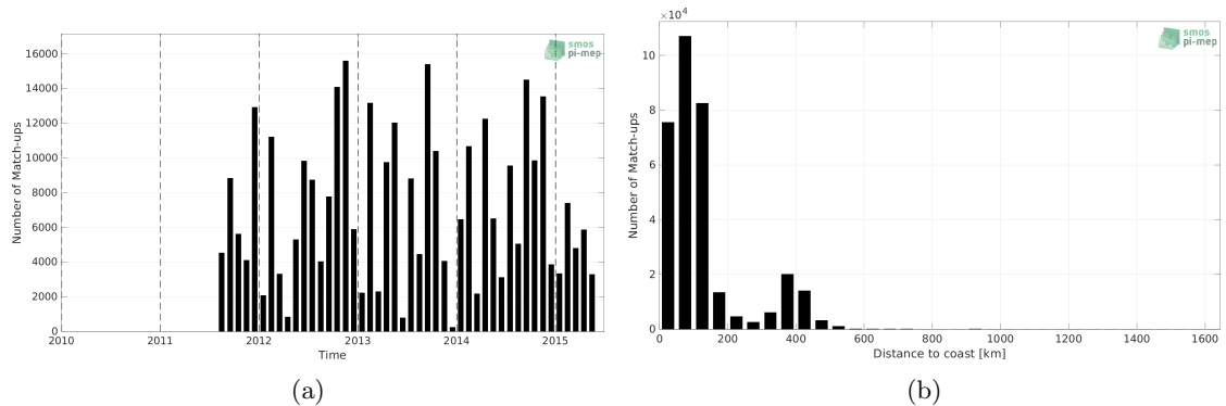
Figure 1: Number of match-ups between ICES and Aquarius SSS L4 OI v5 - Weekly (IPRC) SSS as a function of time (a) and as function of the distance to coast (b) over the North Atlantic Ocean Pi-MEP region and for the full satellite product period.
