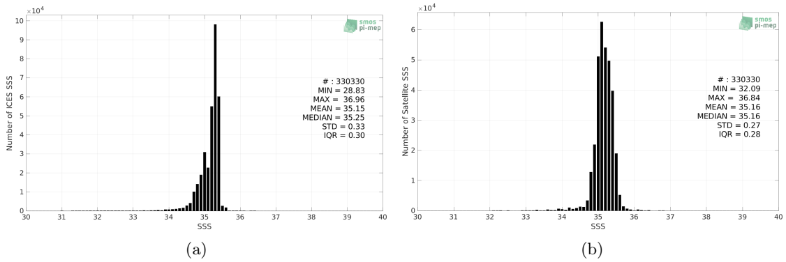
Figure 2: Histograms of SSS from ICES (a) and Aquarius SSS L4 OI v5 - Weekly (IPRC) (b) considering all match-up pairs per bins of 0.1 over the North Atlantic Ocean Pi-MEP region and for the full satellite product period.
