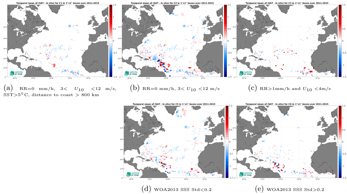
Figure 11: Temporal mean gridded over spatial boxes of size 1^\circ \times 1^\circ of \Delta\text{SSS} (Aquarius SSS L4 OI v5 - Weekly (IPRC) - Surface drifters) for 5 different subdatasets corresponding to:RR=0 mm/h, 3 < U_{10} < 12 m/s, SST >5^\circ\text{C} , distance to coast > 800 km (a), RR=0 mm/h, 3 < U_{10} < 12 m/s (b), RR >1 mm/h and U_{10} < 4 m/s (c), WOA2013 SSS Std <0.2 (d), WOA2013 SSS Std >0.2 (e).
