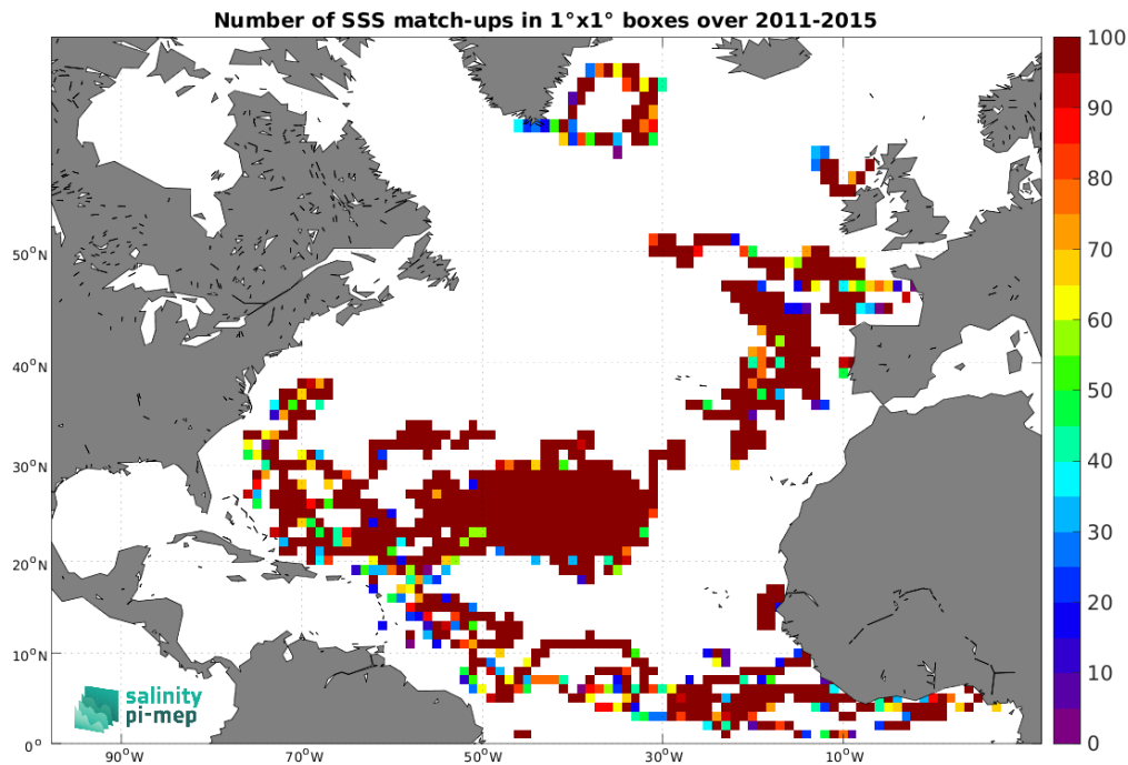
Figure 3: Number of SSS match-ups between Surface drifters SSS and the Aquarius SSS L4 OI v5 - Weekly (IPRC) SSS product for the North Atlantic Ocean Pi-MEP region over 1^{\circ} \times 1^{\circ} boxes and for the full satellite product period.
