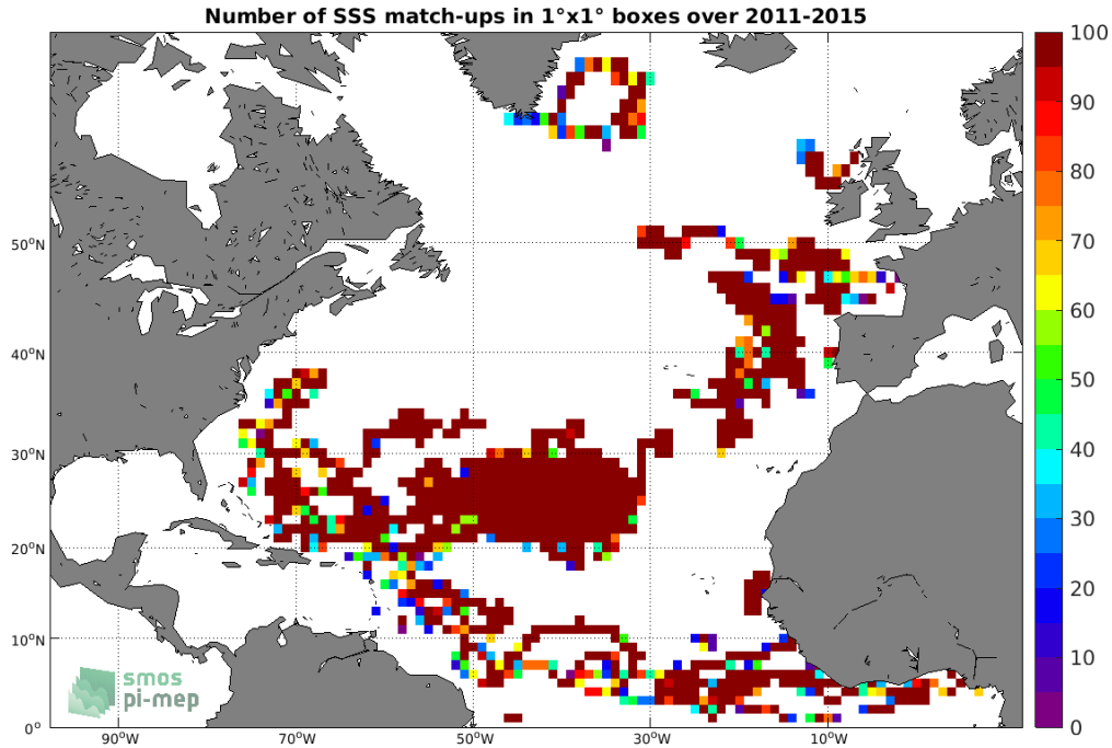
Figure 3: Number of SSS match-ups between Surface drifters SSS and the Aquarius SSS L4 OI v5 - Weekly (IPRC) SSS product for the North Atlantic Ocean Pi-MEP region over 1°x1° boxes and for the full satellite product period.
