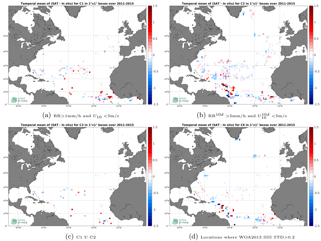
Figure 11: Temporal mean gridded over spatial boxes of size 1^\circ \times 1^\circ of \Delta SSS (Aquarius-L4-IPRC-V5-WEEKLY - Surface drifters) for 4 different subdatasets corresponding to: RR > 1\text{mm/h} and U_{10} < 5\text{m/s} (a), RR^{10d} > 5\text{mm/h} and U_{10}^{10d} < 5\text{m/s} (b), C1 U C2 (c), Locations where WOA2013 SSS STD > 0.2 (d).
