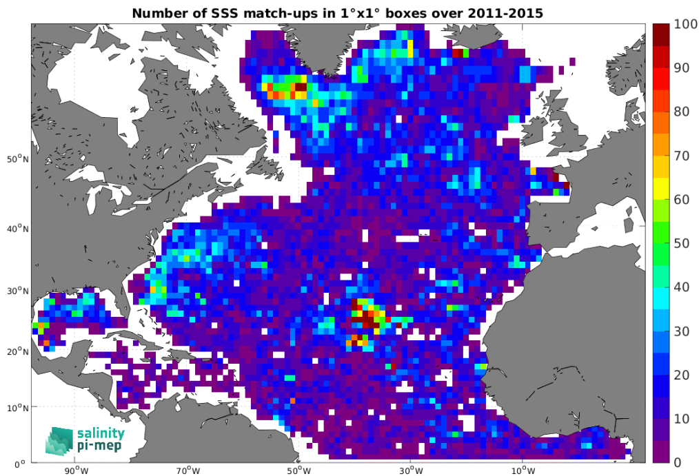
Figure 5: Number of SSS match-ups between Argo SSS and the Aquarius SSS L4 OI v5 - Weekly (IPRC) SSS product for the North Atlantic Ocean Pi-MEP region over 1^\circ \times 1^\circ boxes and for the full satellite product period.
