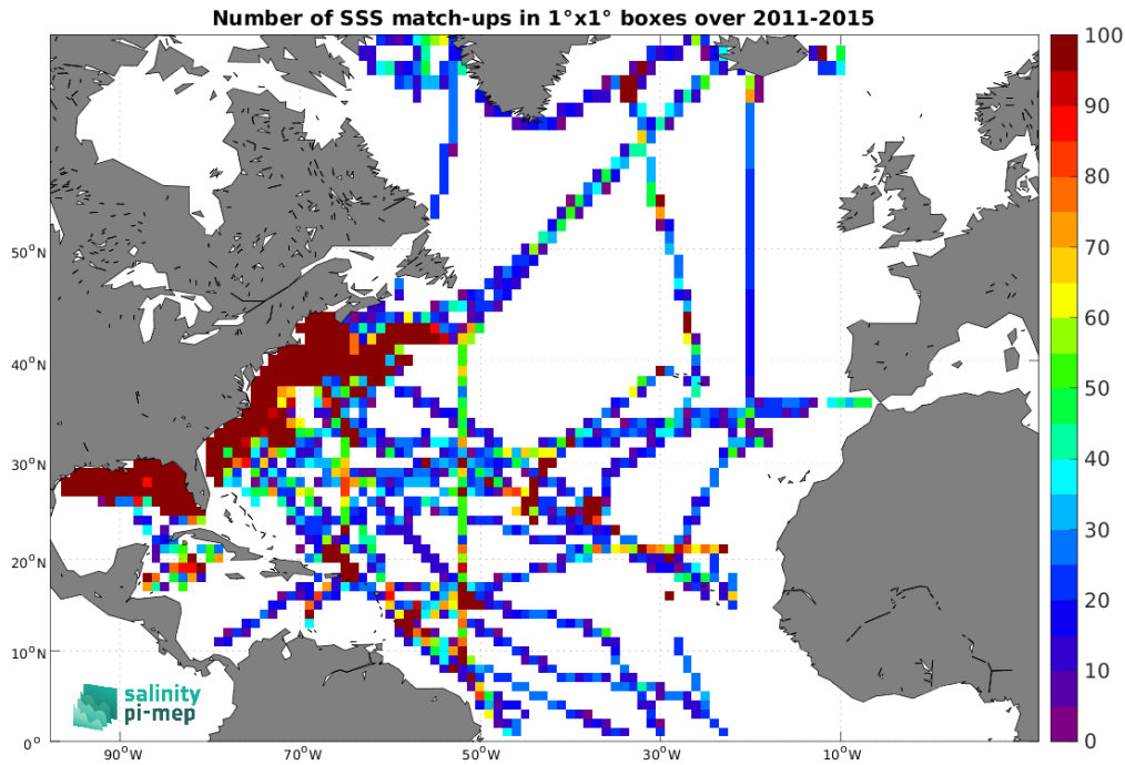
Figure 5: Number of SSS match-ups between TSG (SAMOS) SSS and the Aquarius SSS L4 OI v5 - Monthly (IPRC) SSS product for the North Atlantic Ocean Pi-MEP region over 1^\circ \times 1^\circ boxes and for the full satellite product period.
