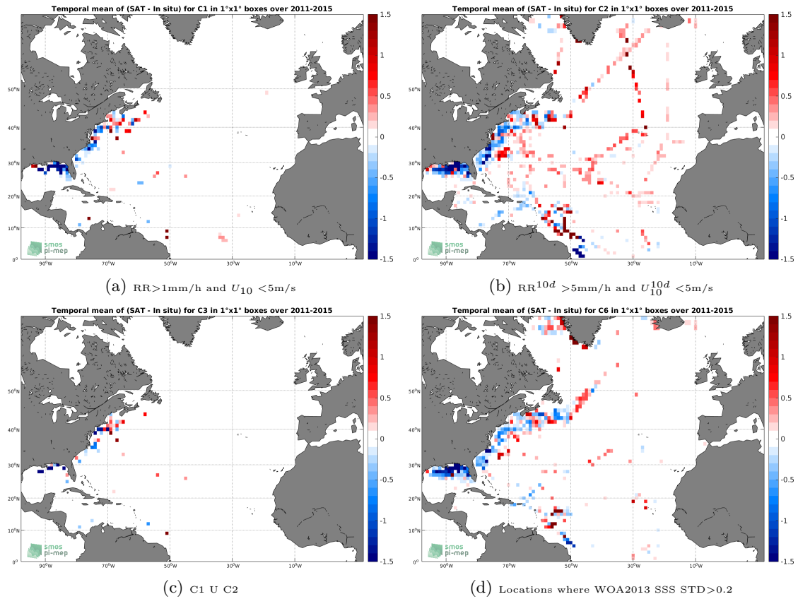
Figure 12: Temporal mean gridded over spatial boxes of size 1^\circ \times 1^\circ of \Delta SSS (Aquarius-L4-IPRC-V5-MONTHLY - TSG-SAMOS) for 4 different subdatasets corresponding to: RR > 1\text{mm/h} and U_{10} < 5\text{m/s} (a), RR^{10d} > 5\text{mm/h} and U_{10}^{10d} < 5\text{m/s} (b), C1 U C2 (c), Locations where WOA2013 SSS STD > 0.2 (d).
