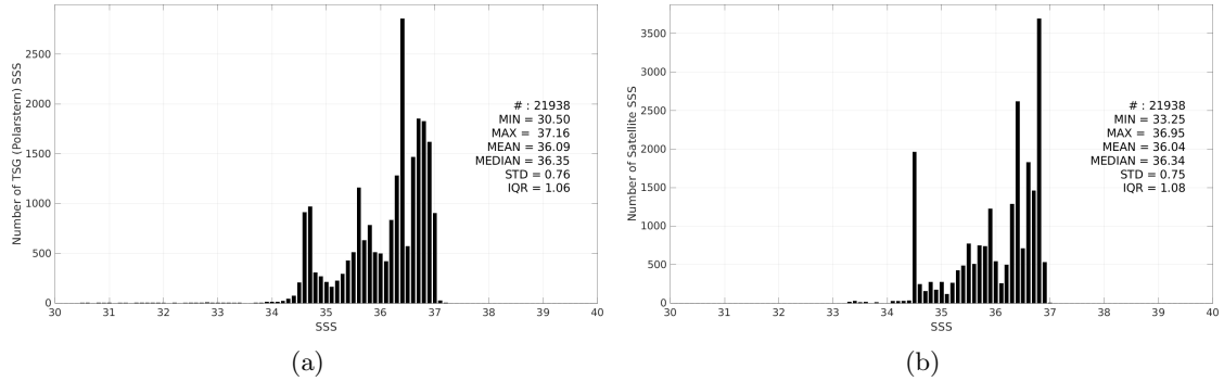
Figure 3: Histograms of SSS from TSG (Polarstern) (a) and Aquarius SSS L4 OI v5 - Monthly (IPRC) (b) considering all match-up pairs per bins of 0.1 over the North Atlantic Ocean Pi-MEP region and for the full satellite product period.
