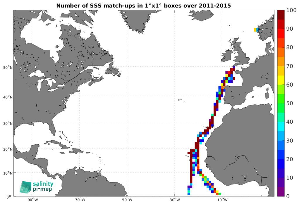
Figure 5: Number of SSS match-ups between TSG (Polarstern) SSS and the Aquarius SSS L4 OI v5 - Monthly (IPRC) SSS product for the North Atlantic Ocean Pi-MEP region over 1^{\circ} \times 1^{\circ} boxes and for the full satellite product period.
