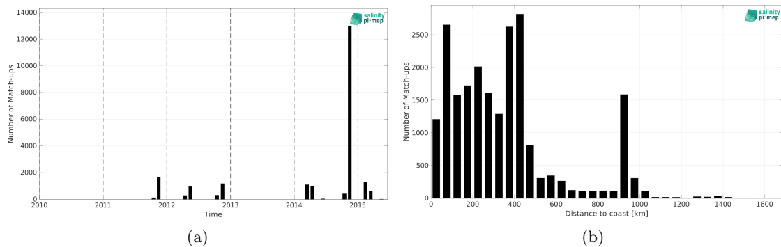
Figure 2: Number of match-ups between TSG (Polarstern) and Aquarius SSS L4 OI v5 - Monthly (IPRC) SSS as a function of time (a) and as function of the distance to coast (b) over the North Atlantic Ocean Pi-MEP region and for the full satellite product period.
