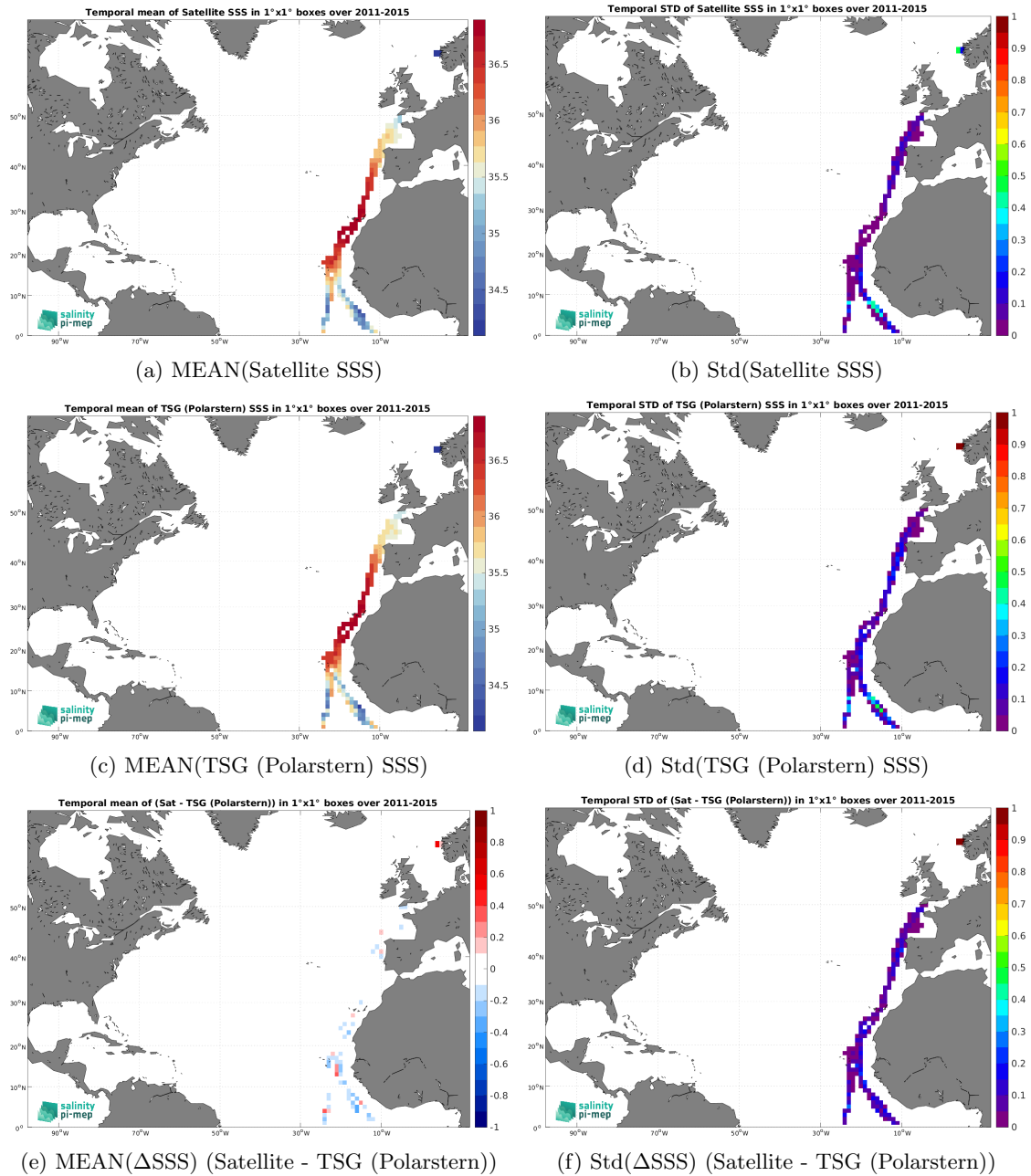
Figure 7: Temporal mean (left) and Std (right) of SSS from Aquarius SSS L4 OI v5 - Monthly (IPRC) (top), TSG (Polarstern) (middle), and of \Delta SSS (Satellite - TSG (Polarstern)). Only match-up pairs are used to generate these maps.
