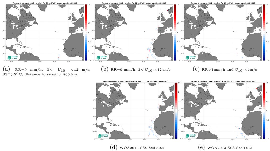
Figure 14: Temporal mean gridded over spatial boxes of size 1^\circ \times 1^\circ of \Delta\text{SSS} (Aquarius SSS L4 OI v5 - Monthly (IPRC) - TSG (Polarstern)) for 5 different subdatasets corresponding to:RR=0 mm/h, 3 < U_{10} < 12 m/s, SST > 5°C, distance to coast > 800 km (a), RR=0 mm/h, 3 < U_{10} < 12 m/s (b), RR > 1mm/h and U_{10} < 4 m/s (c), WOA2013 SSS Std < 0.2 (d), WOA2013 SSS Std > 0.2 (e).
