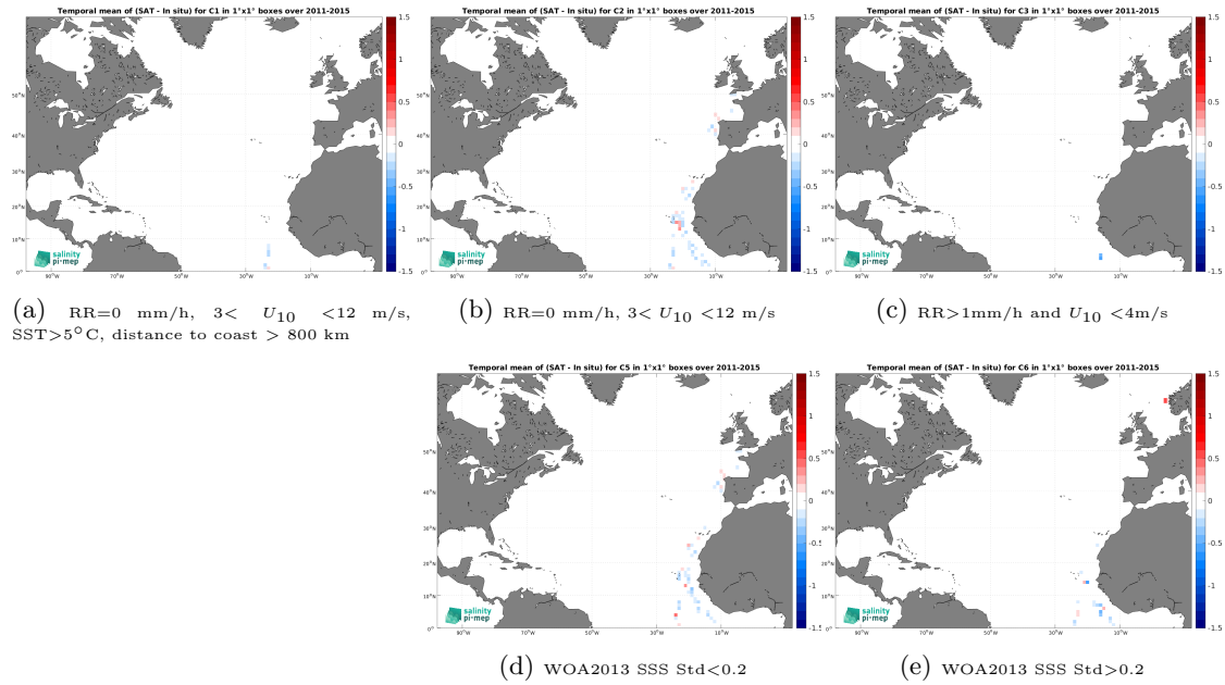
Figure 12: Temporal mean gridded over spatial boxes of size 1^\circ \times 1^\circ of \Delta\text{SSS} (Aquarius SSS L4 OI v5 - Monthly (IPRC) - TSG (Polarstern)) for 5 different subdatasets corresponding to:RR=0 mm/h, 3 < U_{10} < 12 m/s, SST >5^\circ\text{C} , distance to coast > 800 km (a), RR=0 mm/h, 3 < U_{10} < 12 m/s (b), RR >1 mm/h and U_{10} < 4 m/s (c), WOA2013 SSS Std <0.2 (d), WOA2013 SSS Std >0.2 (e).
