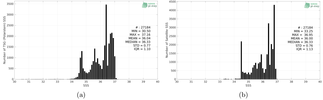
Figure 2: Histograms of SSS from TSG (Polarstern) (a) and Aquarius SSS L4 OI v5 - Monthly (IPRC) (b) considering all match-up pairs per bins of 0.1 over the North Atlantic Ocean Pi-MEP region and for the full satellite product period.
