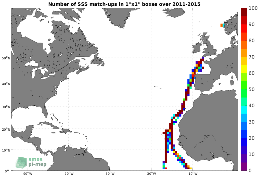
Figure 4: Number of SSS match-ups between TSG (Polarstern) SSS and the Aquarius SSS L4 OI v5 - Monthly (IPRC) SSS product for the North Atlantic Ocean Pi-MEP region over 1^\circ \times 1^\circ boxes and for the full satellite product period.
