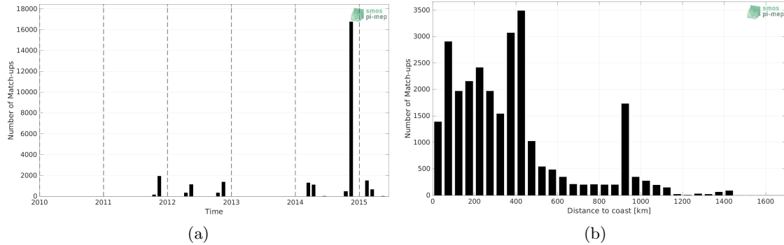
Figure 1: Number of match-ups between TSG (Polarstern) and Aquarius SSS L4 OI v5 - Monthly (IPRC) SSS as a function of time (a) and as function of the distance to coast (b) over the North Atlantic Ocean Pi-MEP region and for the full satellite product period.
