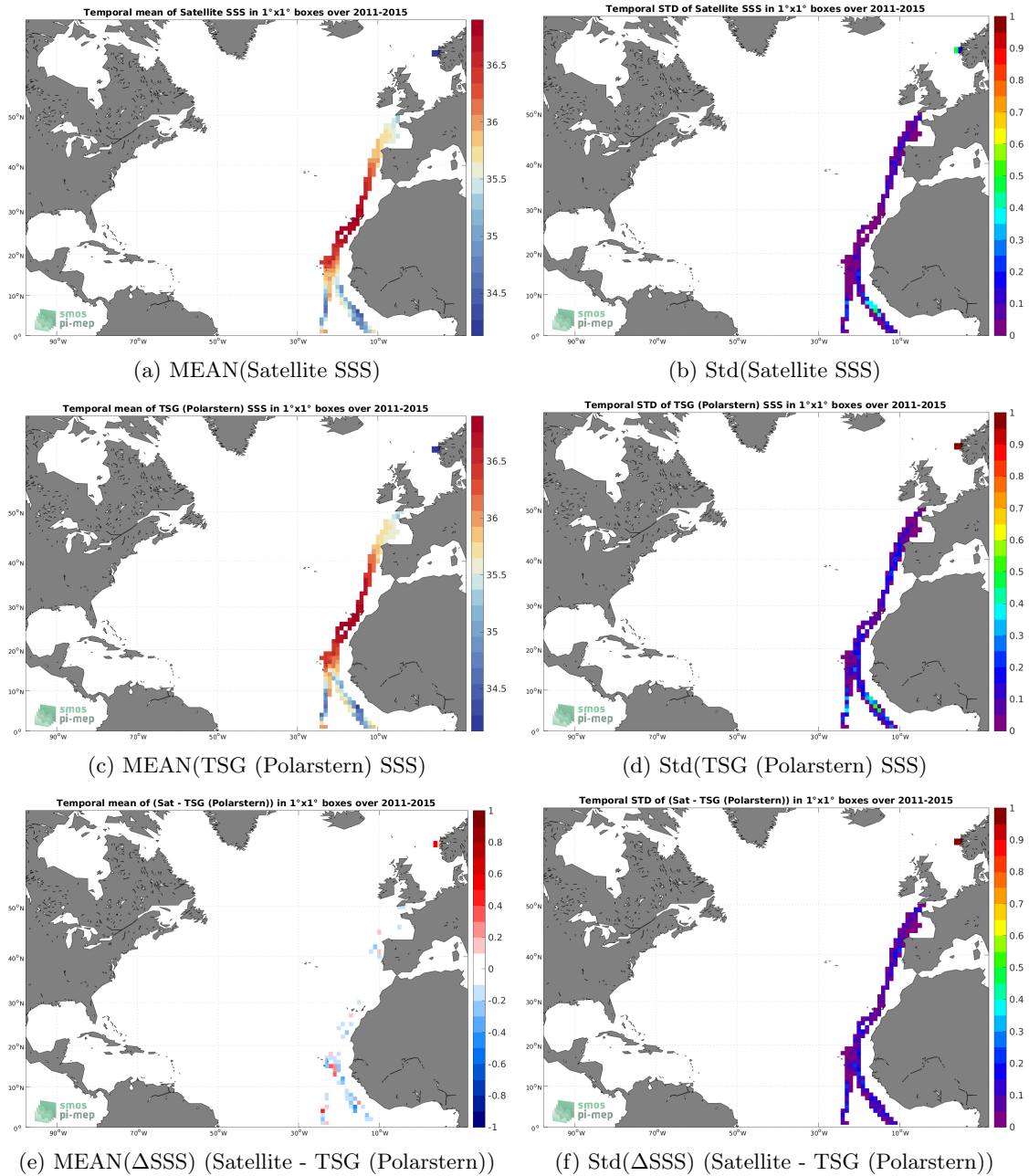
Figure 6: Temporal mean (left) and Std (right) of SSS from Aquarius SSS L4 OI v5 - Monthly (IPRC) (top), TSG (Polarstern) (middle), and of \Delta SSS (Satellite - TSG (Polarstern)). Only match-up pairs are used to generate these maps.
