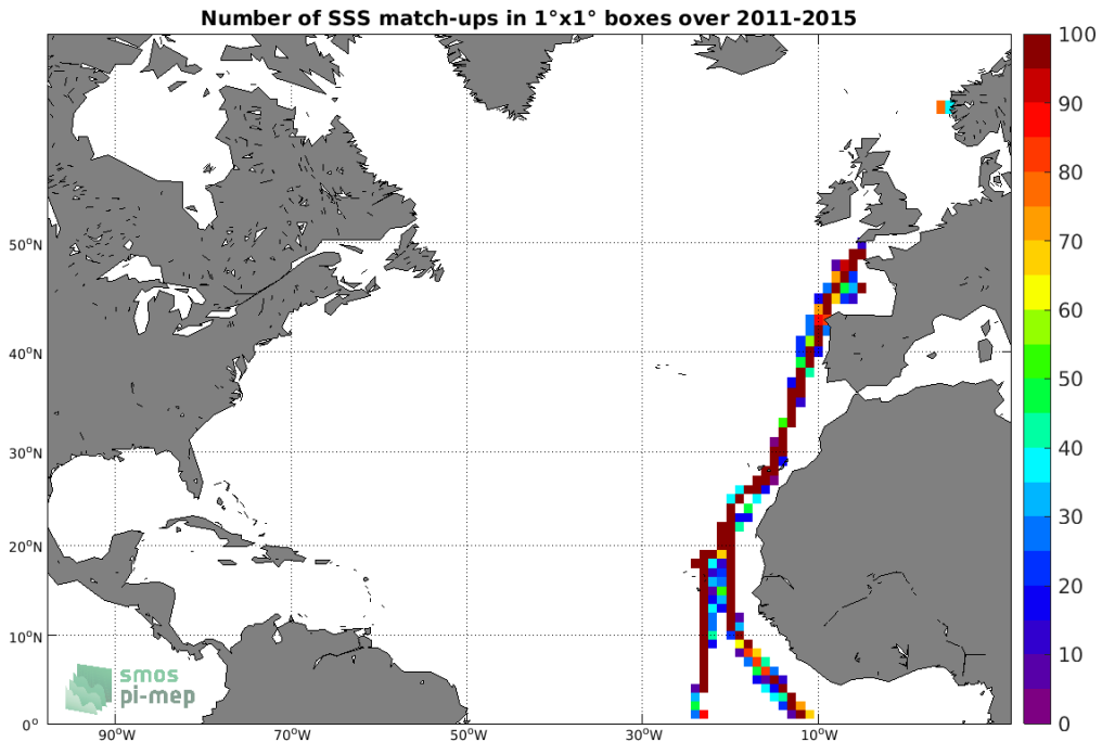
Figure 4: Number of SSS match-ups between TSG (Polarstern) SSS and the Aquarius SSS L4 OI v5 - Monthly (IPRC) SSS product for the North Atlantic Ocean Pi-MEP region over 1°x1° boxes and for the full satellite product period.
