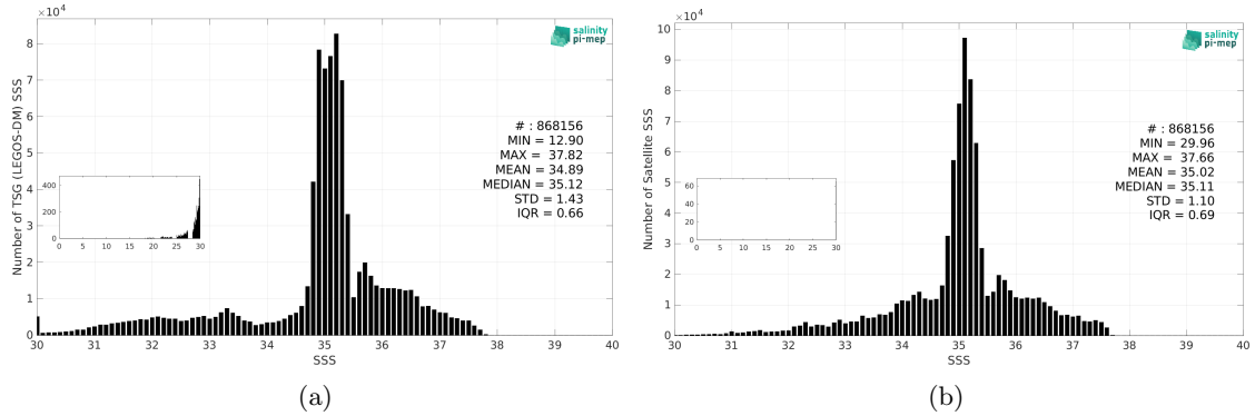
Figure 3: Histograms of SSS from TSG (LEGOS-DM) (a) and Aquarius SSS L4 OI v5 - Monthly (IPRC) (b) considering all match-up pairs per bins of 0.1 over the North Atlantic Ocean Pi-MEP region and for the full satellite product period.
