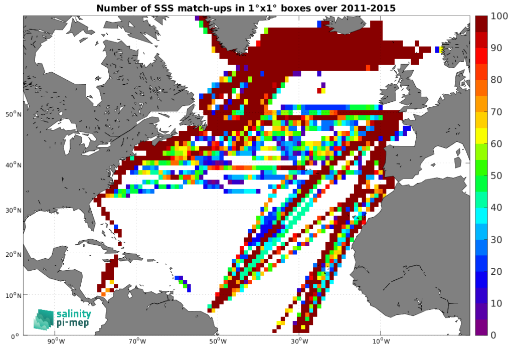
Figure 5: Number of SSS match-ups between TSG (LEGOS-DM) SSS and the Aquarius SSS L4 OI v5 - Monthly (IPRC) SSS product for the North Atlantic Ocean Pi-MEP region over 1^\circ \times 1^\circ boxes and for the full satellite product period.
