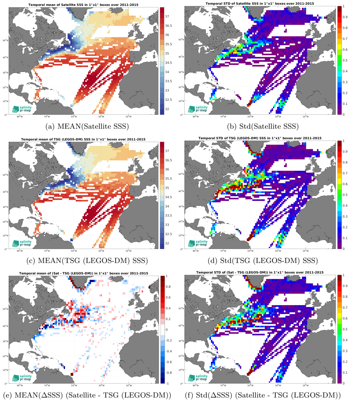
Figure 7: Temporal mean (left) and Std (right) of SSS from Aquarius SSS L4 OI v5 - Monthly (IPRC) (top), TSG (LEGOS-DM) (middle), and of \Delta SSS (Satellite - TSG (LEGOS-DM)). Only match-up pairs are used to generate these maps.
