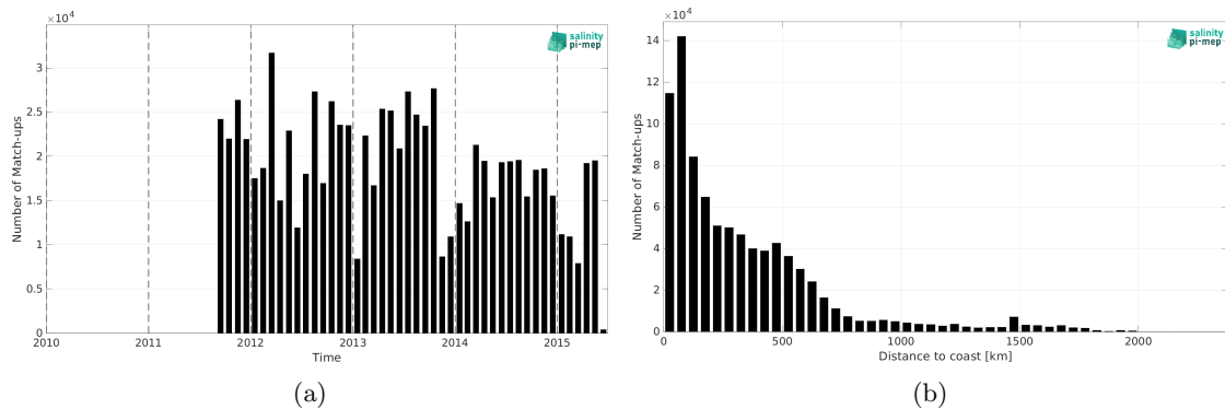
Figure 2: Number of match-ups between TSG (LEGOS-DM) and Aquarius SSS L4 OI v5 - Monthly (IPRC) SSS as a function of time (a) and as function of the distance to coast (b) over the North Atlantic Ocean Pi-MEP region and for the full satellite product period.
