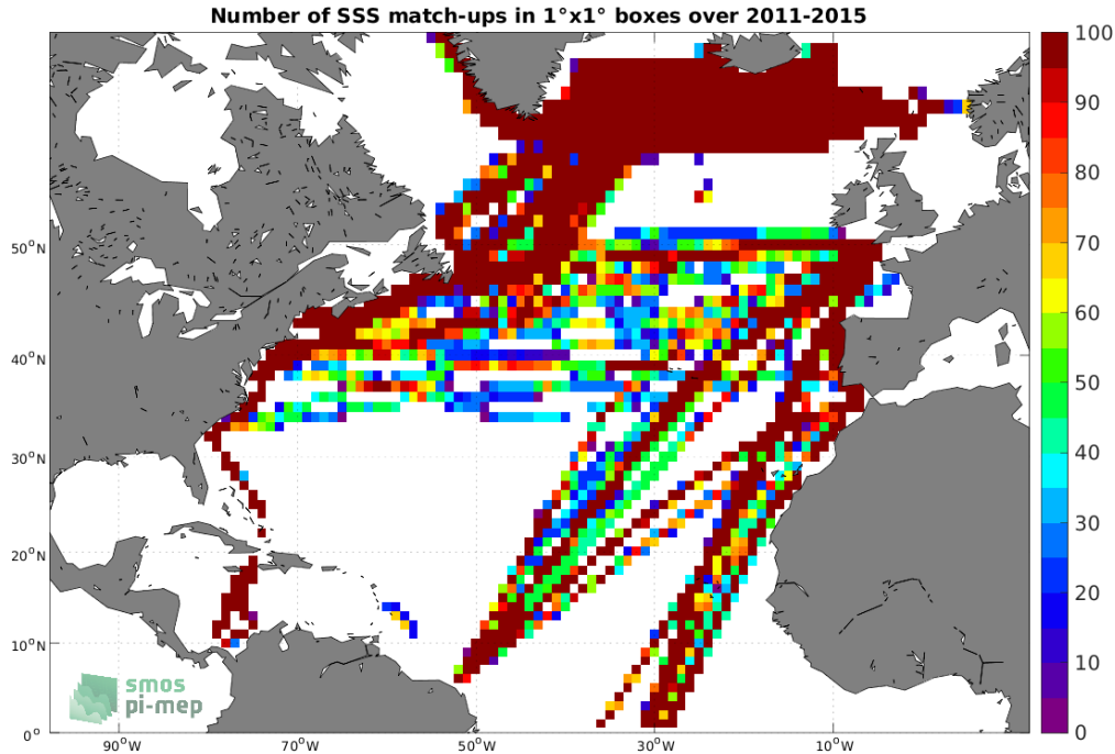
Figure 4: Number of SSS match-ups between TSG (LEGOS-DM) SSS and the Aquarius SSS L4 OI v5 - Monthly (IPRC) SSS product for the North Atlantic Ocean Pi-MEP region over 1^\circ \times 1^\circ boxes and for the full satellite product period.
