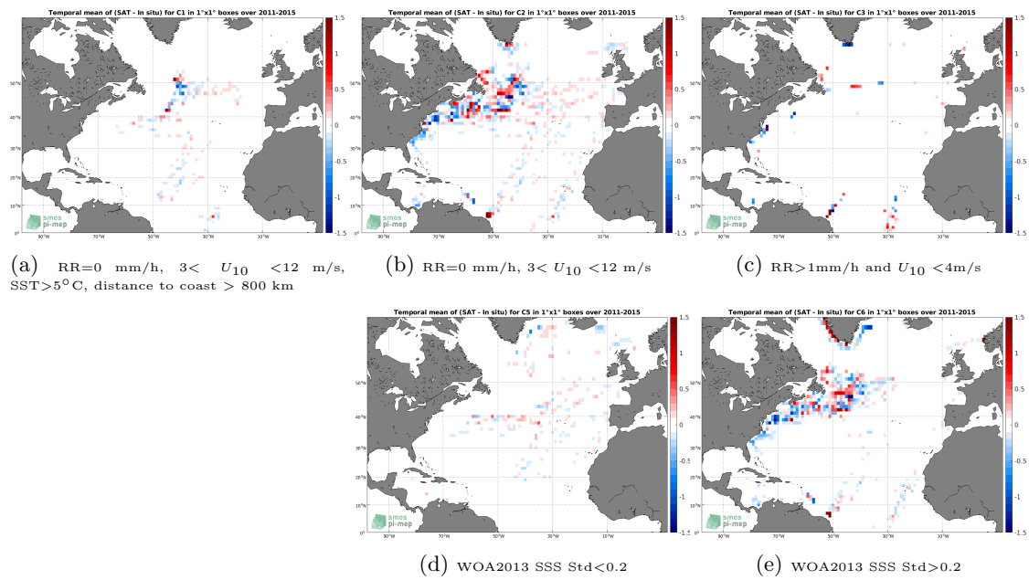
Figure 12: Temporal mean gridded over spatial boxes of size 1^\circ \times 1^\circ of \Delta SSS (Aquarius SSS L4 OI v5 - Monthly (IPRC) - TSG (LEGOS-DM)) for 5 different subdatasets corresponding to:RR=0 mm/h, 3 < U_{10} < 12 m/s, SST >5^\circ C, distance to coast > 800 km (a), RR=0 mm/h, 3 < U_{10} < 12 m/s (b), RR >1 mm/h and U_{10} < 4 m/s (c), WOA2013 SSS Std <0.2 (d), WOA2013 SSS Std >0.2 (e).
