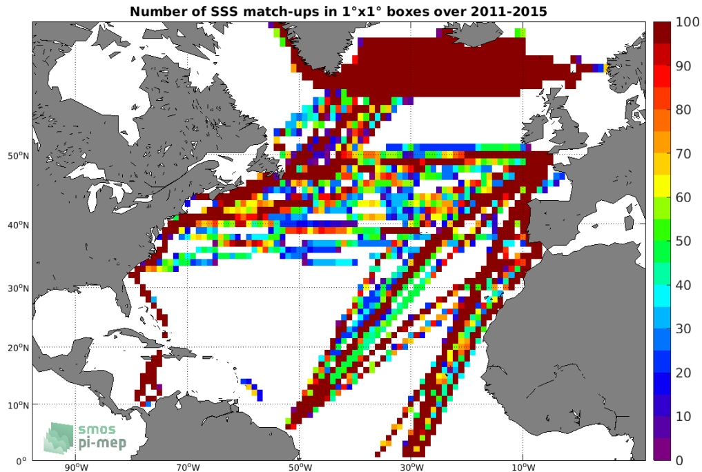
Figure 4: Number of SSS match-ups between TSG (LEGOS-DM) SSS and the Aquarius SSS L4 OI v5 - Monthly (IPRC) SSS product for the North Atlantic Ocean Pi-MEP region over 1°x1° boxes and for the full satellite product period.
