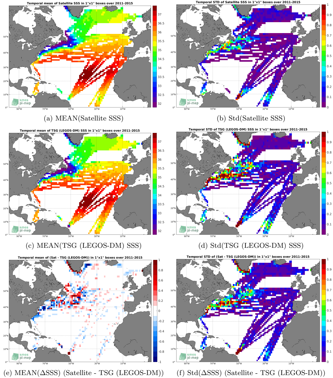
Figure 6: Temporal mean (left) and Std (right) of SSS from Aquarius SSS L4 OI v5 - Monthly (IPRC) (top), TSG (LEGOS-DM) (middle), and of \Delta SSS (Satellite - TSG (LEGOS-DM)). Only match-up pairs are used to generate these maps.
