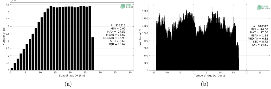
Figure 5: Histograms of the spatial (a) and temporal (b) lags between the time of the TSG (LEGOS-DM) measurements and the date of the corresponding Aquarius SSS L4 OI v5 - Monthly (IPRC) SSS product.
