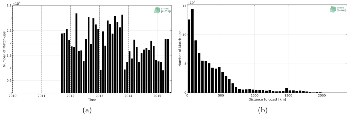
Figure 1: Number of match-ups between TSG (LEGOS-DM) and Aquarius SSS L4 OI v5 - Monthly (IPRC) SSS as a function of time (a) and as function of the distance to coast (b) over the North Atlantic Ocean Pi-MEP region and for the full satellite product period.
