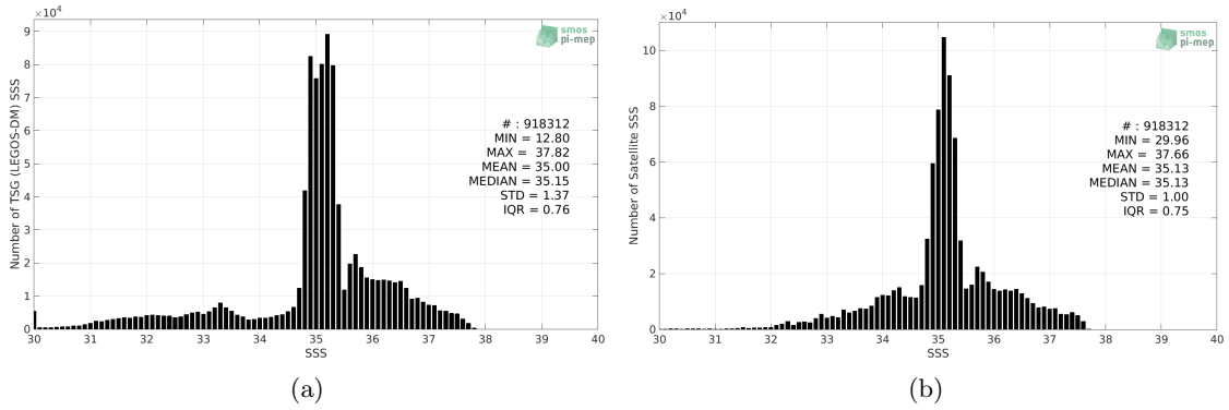
Figure 2: Histograms of SSS from TSG (LEGOS-DM) (a) and Aquarius SSS L4 OI v5 - Monthly (IPRC) (b) considering all match-up pairs per bins of 0.1 over the North Atlantic Ocean Pi-MEP region and for the full satellite product period.
