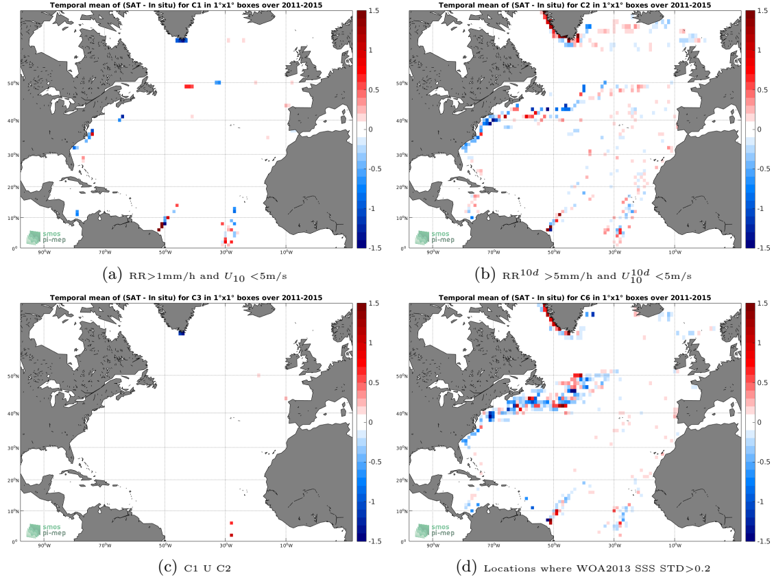
Figure 12: Temporal mean gridded over spatial boxes of size 1^\circ \times 1^\circ of \Delta SSS (Aquarius-L4-IPRC-V5-MONTHLY - TSG-LEGOS-DM) for 4 different subdatasets corresponding to: RR > 1\text{mm/h} and U_{10} < 5\text{m/s} (a), RR^{10d} > 5\text{mm/h} and U_{10}^{10d} < 5\text{m/s} (b), C1 U C2 (c), Locations where WOA2013 SSS STD > 0.2 (d).
