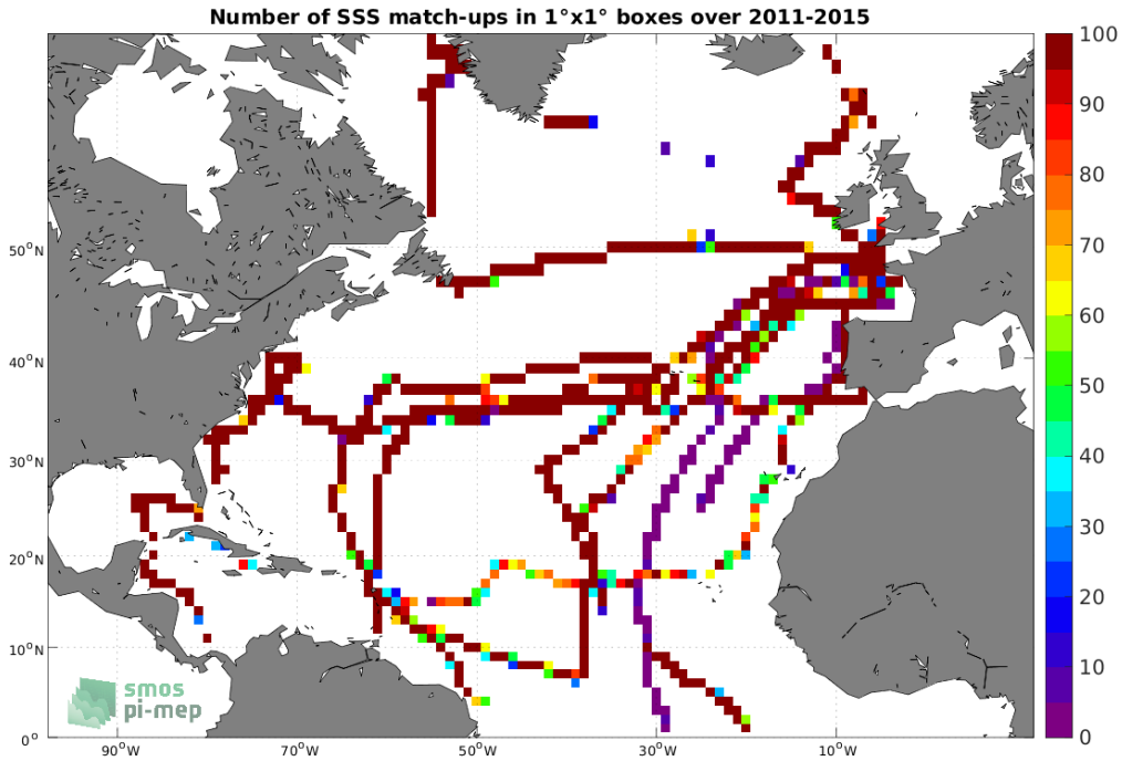
Figure 4: Number of SSS match-ups between TSG (GOSUD-Sailing-ship) SSS and the Aquarius SSS L4 OI v5 - Monthly (IPRC) SSS product for the North Atlantic Ocean Pi-MEP region over 1^\circ \times 1^\circ boxes and for the full satellite product period.
