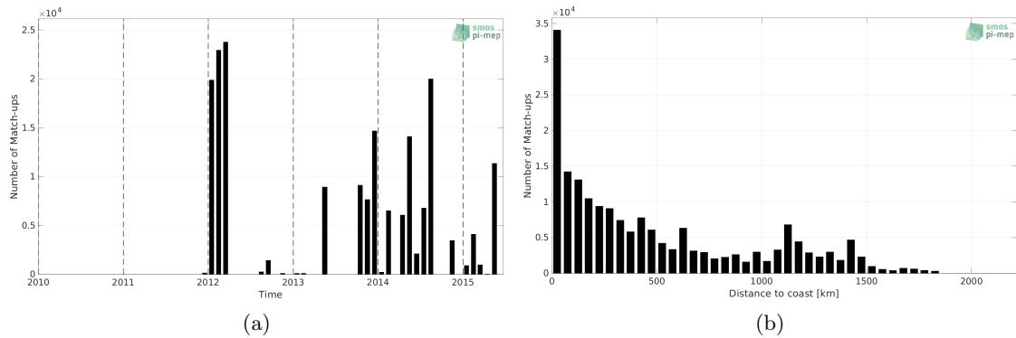
Figure 1: Number of match-ups between TSG (GOSUD-Sailing-ship) and Aquarius SSS L4 OI v5 - Monthly (IPRC) SSS as a function of time (a) and as function of the distance to coast (b) over the North Atlantic Ocean Pi-MEP region and for the full satellite product period.
