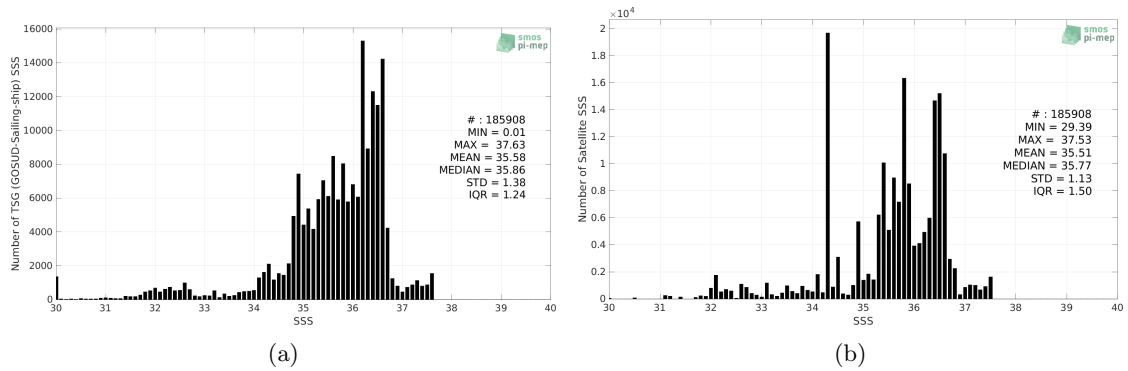
Figure 2: Histograms of SSS from TSG (GOSUD-Sailing-ship) (a) and Aquarius SSS L4 OI v5 - Monthly (IPRC) (b) considering all match-up pairs per bins of 0.1 over the North Atlantic Ocean Pi-MEP region and for the full satellite product period.
