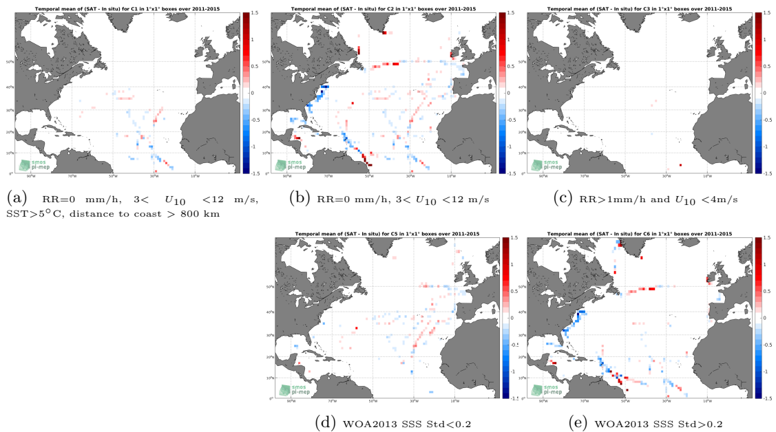
Figure 12: Temporal mean gridded over spatial boxes of size 1^\circ \times 1^\circ of \Delta\text{SSS} (Aquarius SSS L4 OI v5 - Monthly (IPRC) - TSG (GOSUD-Sailing-ship)) for 5 different subdatasets corresponding to:RR=0 mm/h, 3 < U_{10} < 12 m/s, SST>5°C, distance to coast > 800 km (a), RR=0 mm/h, 3 < U_{10} < 12 m/s (b), RR>1mm/h and U_{10} < 4 m/s (c), WOA2013 SSS Std<0.2 (d), WOA2013 SSS Std>0.2 (e).
