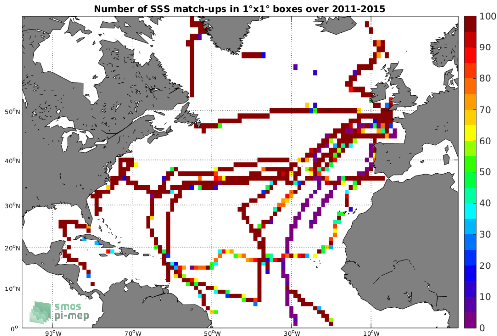
Figure 4: Number of SSS match-ups between TSG-GOSUD-Sailing-ship SSS and the Aquarius-L4-IPRC-V5-MONTHLY SSS product for the North Atlantic Ocean Pi-MEP region over 1°x1° boxes and for the full satellite product period.
