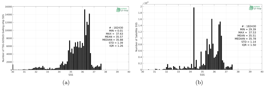
Figure 2: Histograms of SSS from TSG-GOSUD-Sailing-ship (a) and Aquarius-L4-IPRC-V5-MONTHLY (b) considering all match-up pairs per bins of 0.1 over the North Atlantic Ocean Pi-MEP region and for the full satellite product period.
