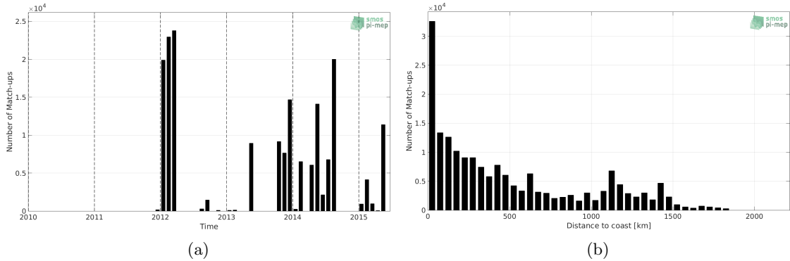
Figure 1: Number of match-ups between TSG-GOSUD-Sailing-ship and Aquarius-L4-IPRC-V5-MONTHLY SSS as a function of time (a) and as function of the distance to coast (b) over the North Atlantic Ocean Pi-MEP region and for the full satellite product period.
