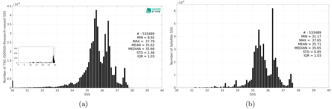
Figure 3: Histograms of SSS from TSG (GOSUD-Research-vessel) (a) and Aquarius SSS L4 OI v5 - Monthly (IPRC) (b) considering all match-up pairs per bins of 0.1 over the North Atlantic Ocean Pi-MEP region and for the full satellite product period.
