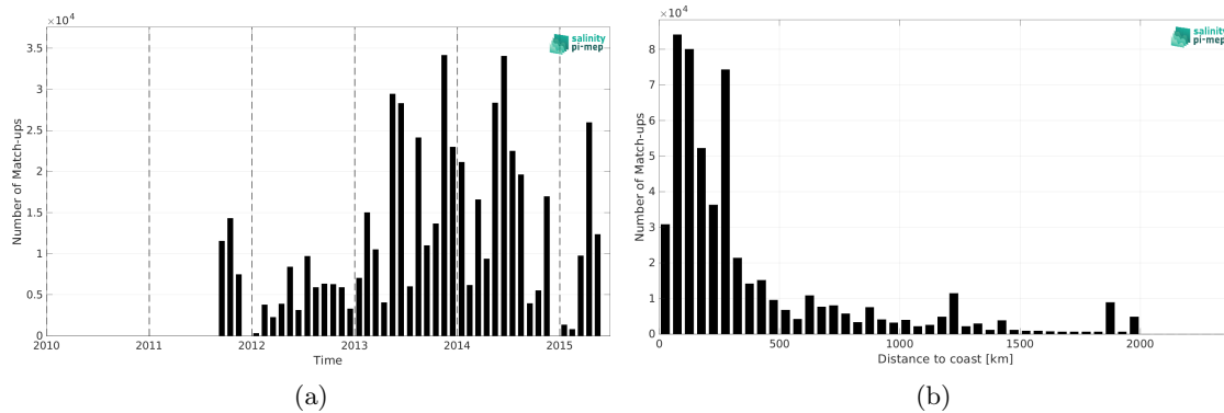
Figure 2: Number of match-ups between TSG (GOSUD-Research-vessel) and Aquarius SSS L4 OI v5 - Monthly (IPRC) SSS as a function of time (a) and as function of the distance to coast (b) over the North Atlantic Ocean Pi-MEP region and for the full satellite product period.
