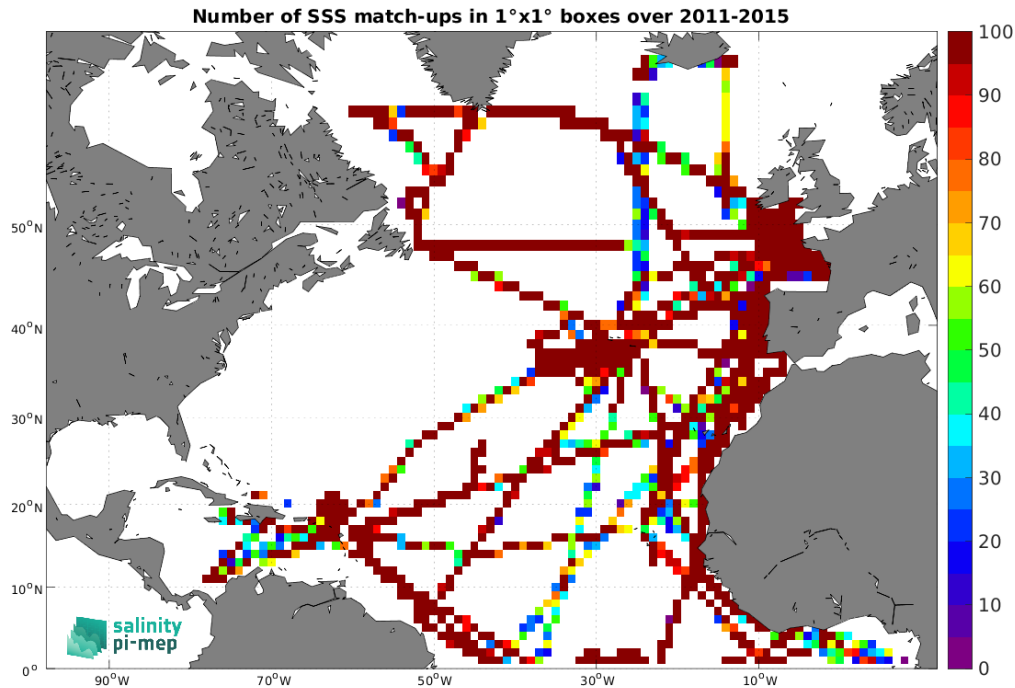
Figure 5: Number of SSS match-ups between TSG (GOSUD-Research-vessel) SSS and the Aquarius SSS L4 OI v5 - Monthly (IPRC) SSS product for the North Atlantic Ocean Pi-MEP region over 1^\circ \times 1^\circ boxes and for the full satellite product period.
