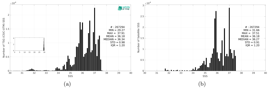
Figure 3: Histograms of SSS from TSG (CSIC-UTM) (a) and Aquarius SSS L4 OI v5 - Monthly (IPRC) (b) considering all match-up pairs per bins of 0.1 over the North Atlantic Ocean Pi-MEP region and for the full satellite product period.
