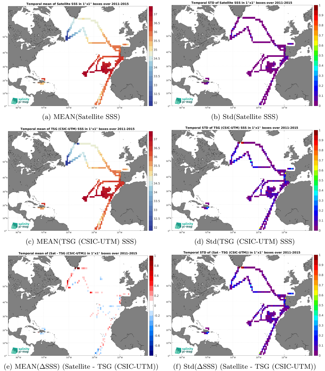
Figure 7: Temporal mean (left) and Std (right) of SSS from Aquarius SSS L4 OI v5 - Monthly (IPRC) (top), TSG (CSIC-UTM) (middle), and of \Delta SSS (Satellite - TSG (CSIC-UTM)). Only match-up pairs are used to generate these maps.
