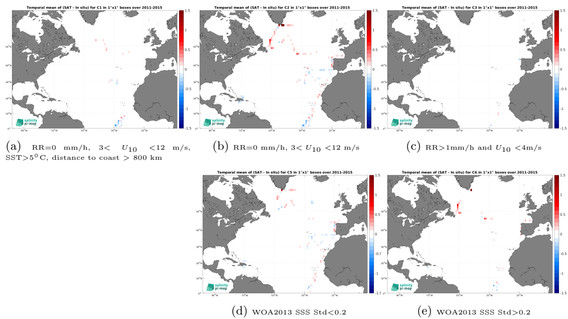
Figure 14: Temporal mean gridded over spatial boxes of size 1^\circ \times 1^\circ of \Delta SSS (Aquarius SSS L4 OI v5 - Monthly (IPRC) - TSG (CSIC-UTM)) for 5 different subdatasets corresponding to:RR=0 mm/h, 3 < U_{10} < 12 m/s, SST >5^\circ\text{C} , distance to coast > 800 km (a), RR=0 mm/h, 3 < U_{10} < 12 m/s (b), RR >1 mm/h and U_{10} < 4 m/s (c), WOA2013 SSS Std <0.2 (d), WOA2013 SSS Std >0.2 (e).
