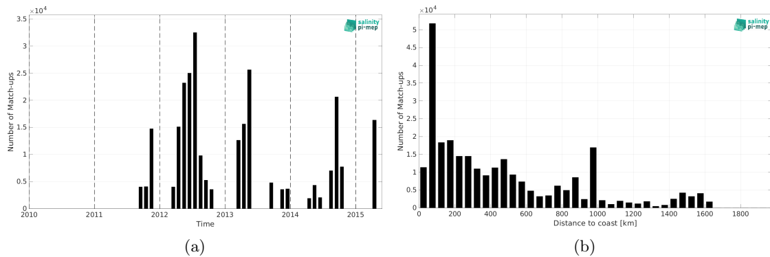
Figure 2: Number of match-ups between TSG (CSIC-UTM) and Aquarius SSS L4 OI v5 - Monthly (IPRC) SSS as a function of time (a) and as function of the distance to coast (b) over the North Atlantic Ocean Pi-MEP region and for the full satellite product period.
