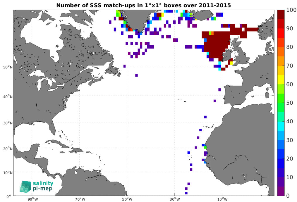
Figure 5: Number of SSS match-ups between ICES SSS and the Aquarius SSS L4 OI v5 - Monthly (IPRC) SSS product for the North Atlantic Ocean Pi-MEP region over 1^\circ \times 1^\circ boxes and for the full satellite product period.
