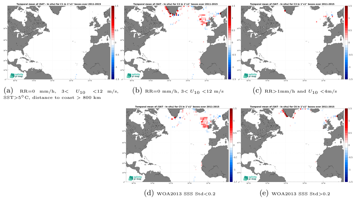
Figure 14: Temporal mean gridded over spatial boxes of size 1^\circ \times 1^\circ of \Delta SSS (Aquarius SSS L4 OI v5 - Monthly (IPRC) - ICES) for 5 different subdatasets corresponding to:RR=0 mm/h, 3 < U_{10} < 12 m/s, SST > 5°C, distance to coast > 800 km (a), RR=0 mm/h, 3 < U_{10} < 12 m/s (b), RR > 1mm/h and U_{10} < 4 m/s (c), WOA2013 SSS Std < 0.2 (d), WOA2013 SSS Std > 0.2 (e).
