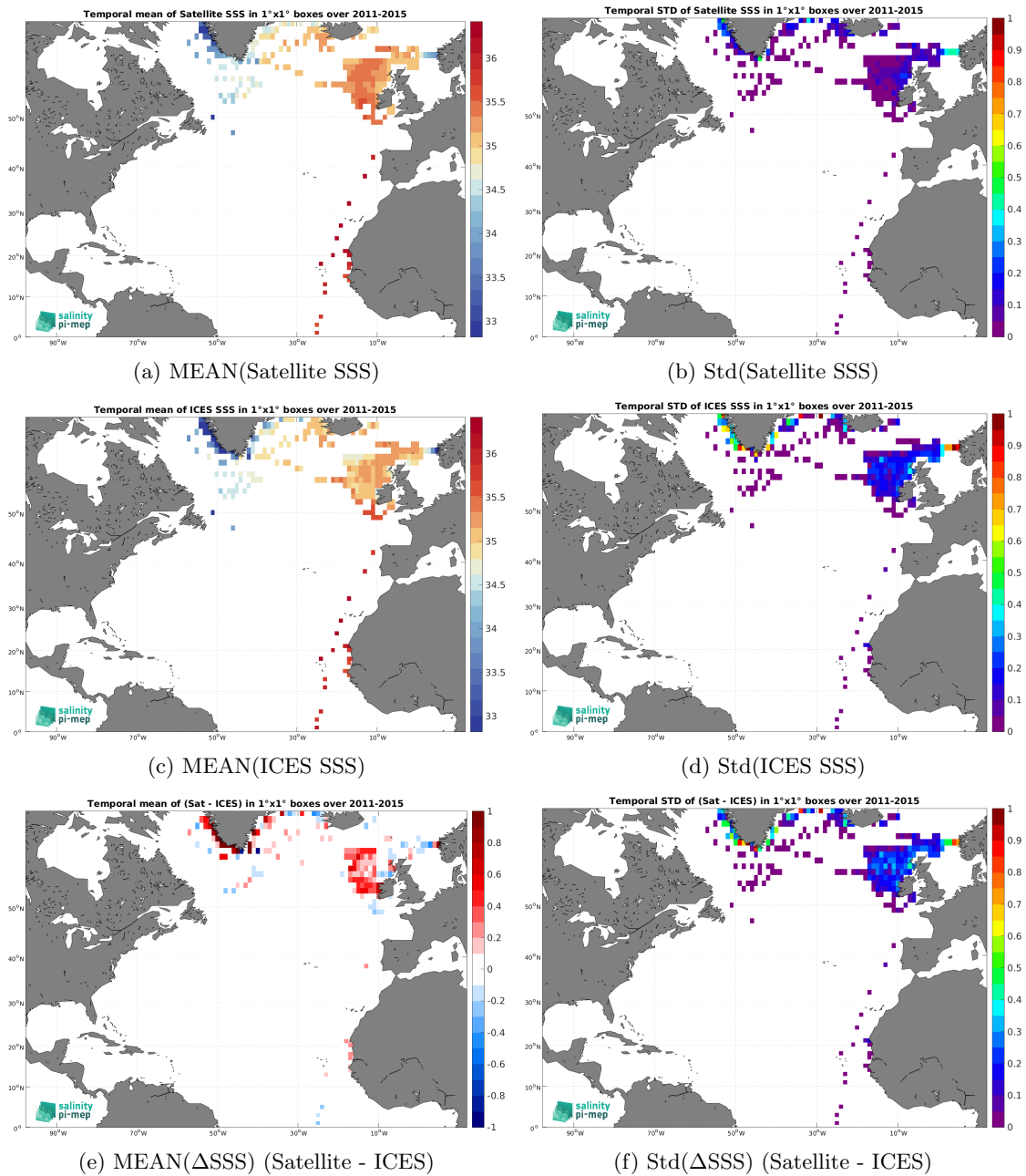
Figure 7: Temporal mean (left) and Std (right) of SSS from Aquarius SSS L4 OI v5 - Monthly (IPRC) (top), ICES (middle), and of \Delta SSS (Satellite - ICES). Only match-up pairs are used to generate these maps.
