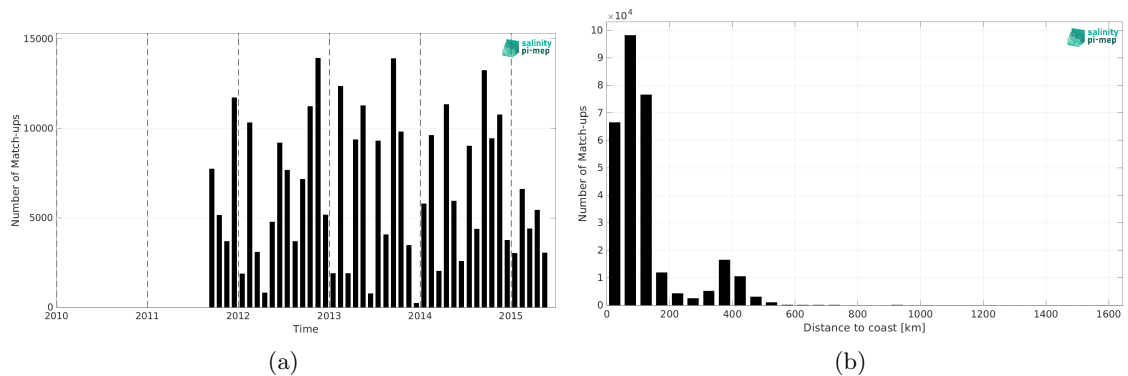
Figure 2: Number of match-ups between ICES and Aquarius SSS L4 OI v5 - Monthly (IPRC) SSS as a function of time (a) and as function of the distance to coast (b) over the North Atlantic Ocean Pi-MEP region and for the full satellite product period.
