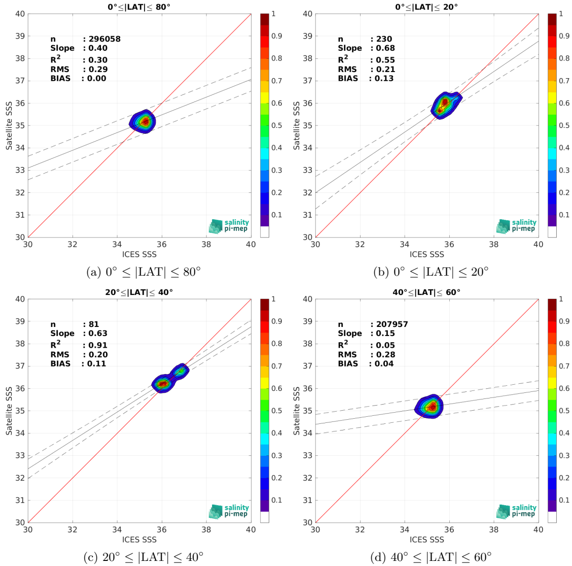
Figure 10: Contour maps of the concentration of Aquarius SSS L4 OI v5 - Monthly (IPRC) SSS (y-axis) versus ICES SSS (x-axis) at match-up pairs for different latitude bands. For each plot, the red line shows x=y . The black thin and dashed lines indicate a linear fit through the data cloud and the \pm 95\% confidence levels, respectively. The number match-up pairs n , the slope and R^2 coefficient of the linear fit, the root mean square (RMS) and the mean bias between satellite and in situ data are indicated for each latitude band in each plots.
