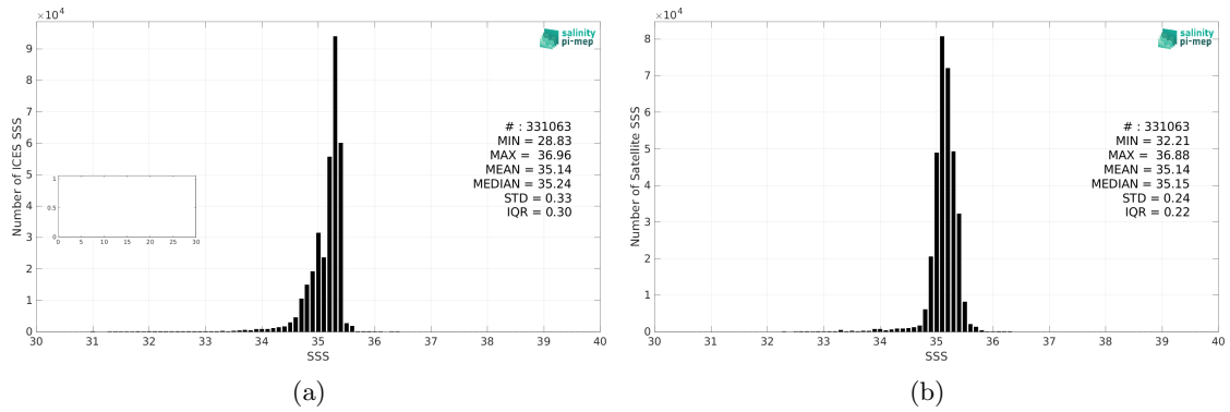
Figure 2: Histograms of SSS from ICES (a) and Aquarius SSS L4 OI v5 - Monthly (IPRC) (b) considering all match-up pairs per bins of 0.1 over the North Atlantic Ocean Pi-MEP region and for the full satellite product period.
