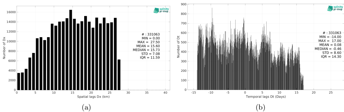
Figure 5: Histograms of the spatial (a) and temporal (b) lags between the location/time of the ICES measurement and the date of the corresponding Aquarius SSS L4 OI v5 - Monthly (IPRC) SSS pixel.
