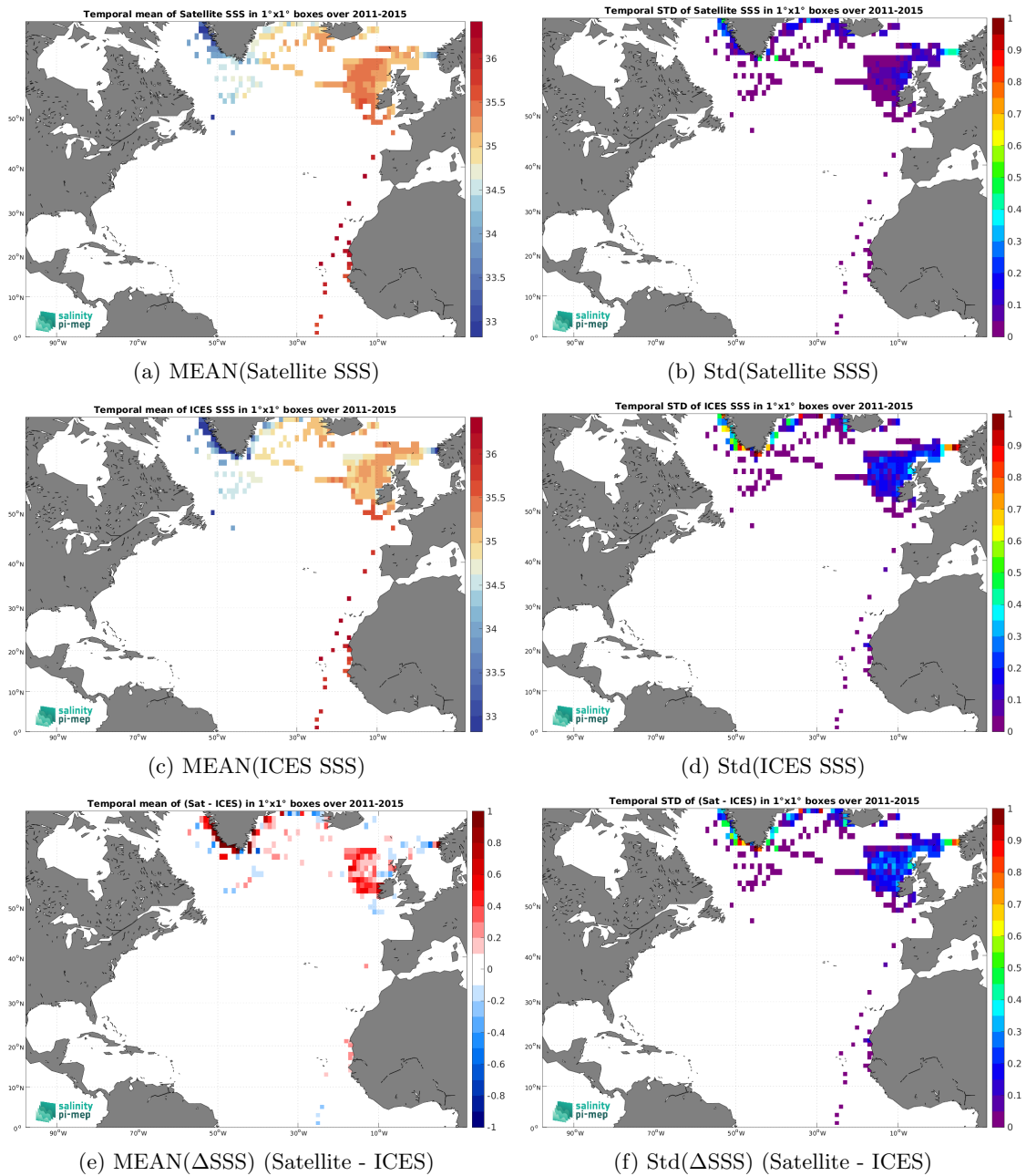
Figure 6: Temporal mean (left) and Std (right) of SSS from Aquarius SSS L4 OI v5 - Monthly (IPRC) (top), ICES (middle), and of \Delta SSS (Satellite - ICES). Only match-up pairs are used to generate these maps.
