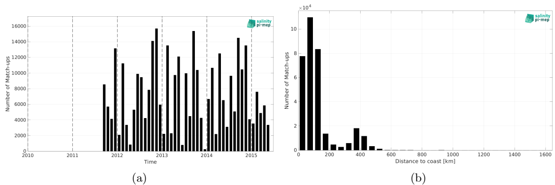
Figure 1: Number of match-ups between ICES and Aquarius SSS L4 OI v5 - Monthly (IPRC) SSS as a function of time (a) and as function of the distance to coast (b) over the North Atlantic Ocean Pi-MEP region and for the full satellite product period.
