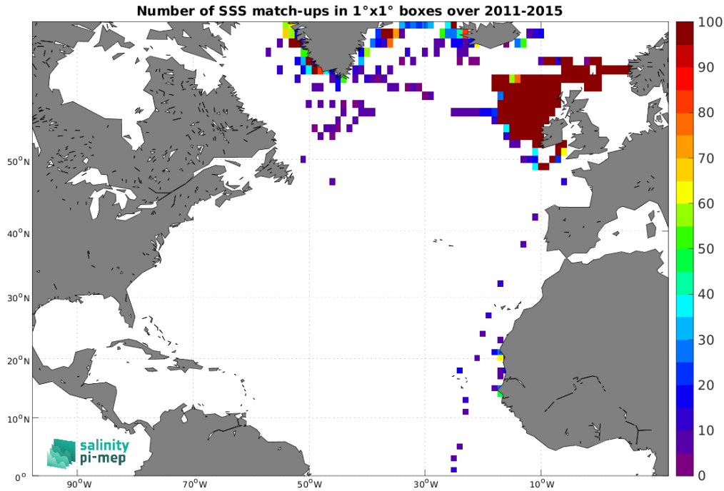
Figure 4: Number of SSS match-ups between ICES SSS and the Aquarius SSS L4 OI v5 - Monthly (IPRC) SSS product for the North Atlantic Ocean Pi-MEP region over 1^{\circ} \times 1^{\circ} boxes and for the full satellite product period.
