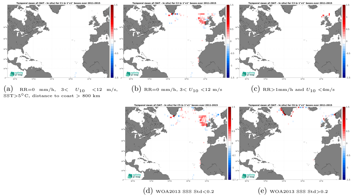
Figure 12: Temporal mean gridded over spatial boxes of size 1^\circ \times 1^\circ of \Delta SSS (Aquarius SSS L4 OI v5 - Monthly (IPRC) - ICES) for 5 different subdatasets corresponding to:RR=0 mm/h, 3 < U_{10} < 12 m/s, SST >5^\circ\text{C} , distance to coast > 800 km (a), RR=0 mm/h, 3 < U_{10} < 12 m/s (b), RR >1 mm/h and U_{10} < 4 m/s (c), WOA2013 SSS Std <0.2 (d), WOA2013 SSS Std >0.2 (e).
