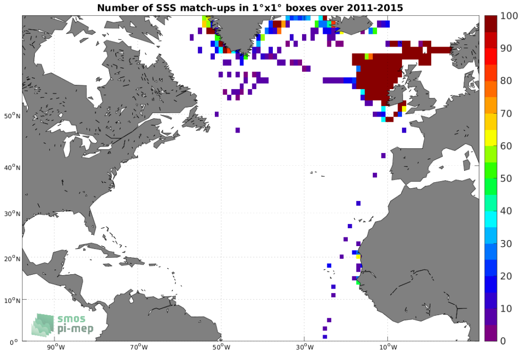
Figure 4: Number of SSS match-ups between ICES SSS and the Aquarius SSS L4 OI v5 - Monthly (IPRC) SSS product for the North Atlantic Ocean Pi-MEP region over 1^\circ \times 1^\circ boxes and for the full satellite product period.
