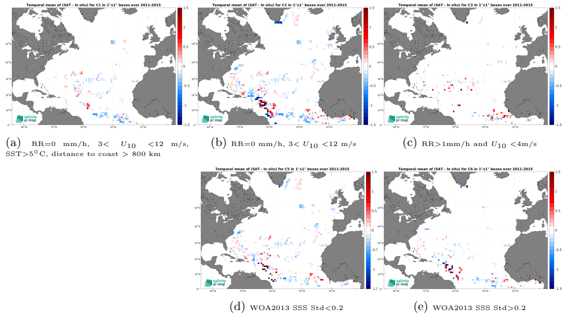
Figure 13: Temporal mean gridded over spatial boxes of size 1^\circ \times 1^\circ of \Delta\text{SSS} (Aquarius SSS L4 OI v5 - Monthly (IPRC) - Surface drifters) for 5 different subdatasets corresponding to:RR=0 mm/h, 3 < U_{10} < 12 m/s, SST >5^\circ\text{C} , distance to coast > 800 km (a), RR=0 mm/h, 3 < U_{10} < 12 m/s (b), RR >1 mm/h and U_{10} < 4 m/s (c), WOA2013 SSS Std <0.2 (d), WOA2013 SSS Std >0.2 (e).
