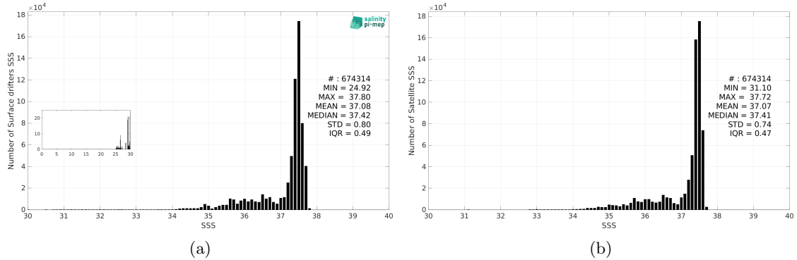
Figure 3: Histograms of SSS from Surface drifters (a) and Aquarius SSS L4 OI v5 - Monthly (IPRC) (b) considering all match-up pairs per bins of 0.1 over the North Atlantic Ocean Pi-MEP region and for the full satellite product period.
