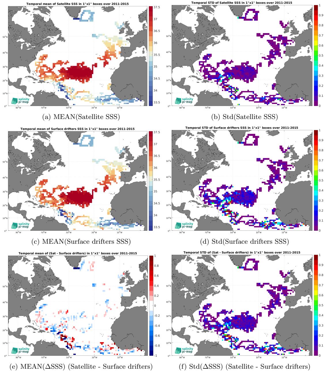
Figure 6: Temporal mean (left) and Std (right) of SSS from Aquarius SSS L4 OI v5 - Monthly (IPRC) (top), Surface drifters (middle), and of \Delta SSS (Satellite - Surface drifters). Only match-up pairs are used to generate these maps.
