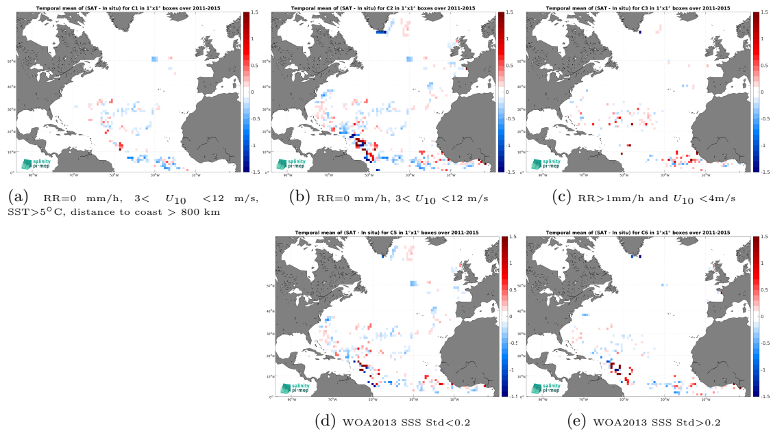
Figure 13: Temporal mean gridded over spatial boxes of size 1^\circ \times 1^\circ of \Delta SSS (Aquarius SSS L4 OI v5 - Monthly (IPRC) - Surface drifters) for 5 different subdatasets corresponding to:RR=0 mm/h, 3 < U_{10} < 12 m/s, SST >5^\circ\text{C} , distance to coast > 800 km (a), RR=0 mm/h, 3 < U_{10} < 12 m/s (b), RR >1 mm/h and U_{10} < 4 m/s (c), WOA2013 SSS Std <0.2 (d), WOA2013 SSS Std >0.2 (e).
