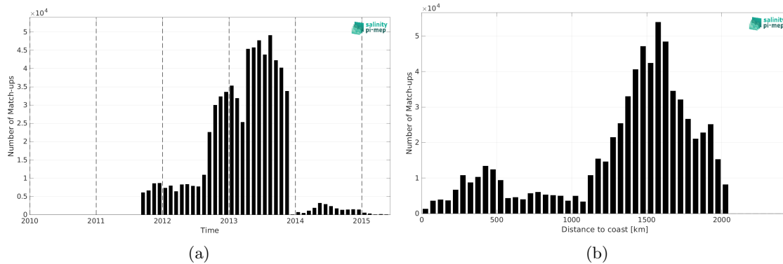
Figure 2: Number of match-ups between Surface drifters and Aquarius SSS L4 OI v5 - Monthly (IPRC) SSS as a function of time (a) and as function of the distance to coast (b) over the North Atlantic Ocean Pi-MEP region and for the full satellite product period.
