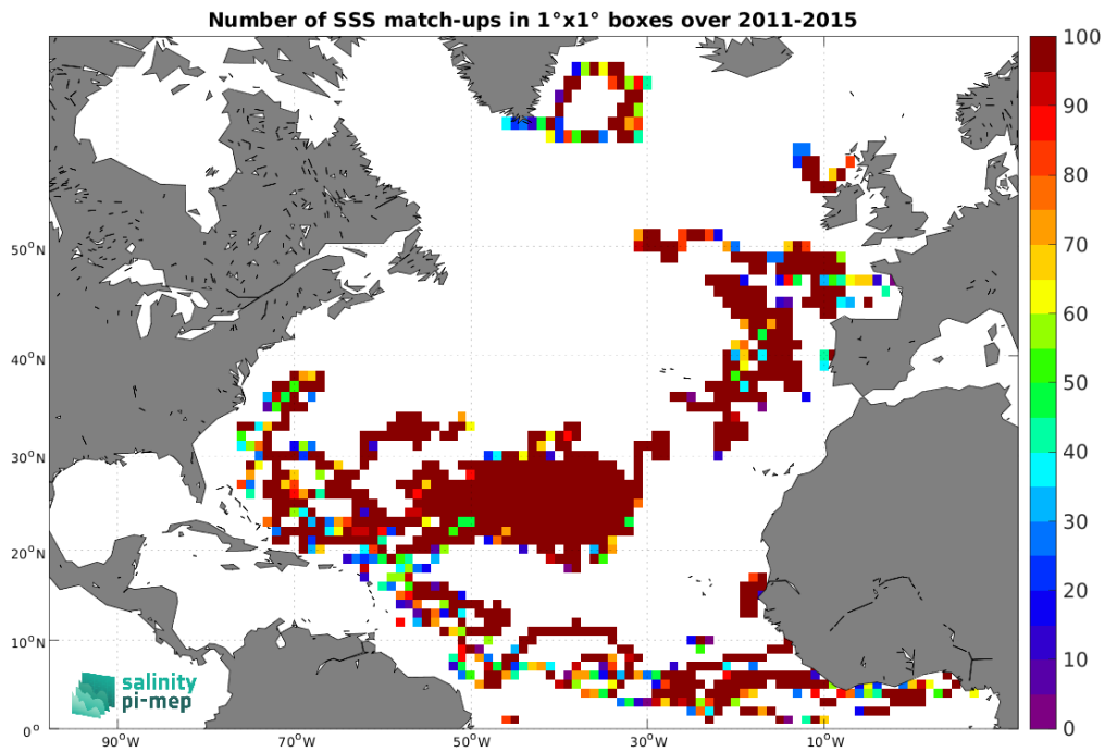
Figure 4: Number of SSS match-ups between Surface drifters SSS and the Aquarius SSS L4 OI v5 - Monthly (IPRC) SSS product for the North Atlantic Ocean Pi-MEP region over 1^\circ \times 1^\circ boxes and for the full satellite product period.
