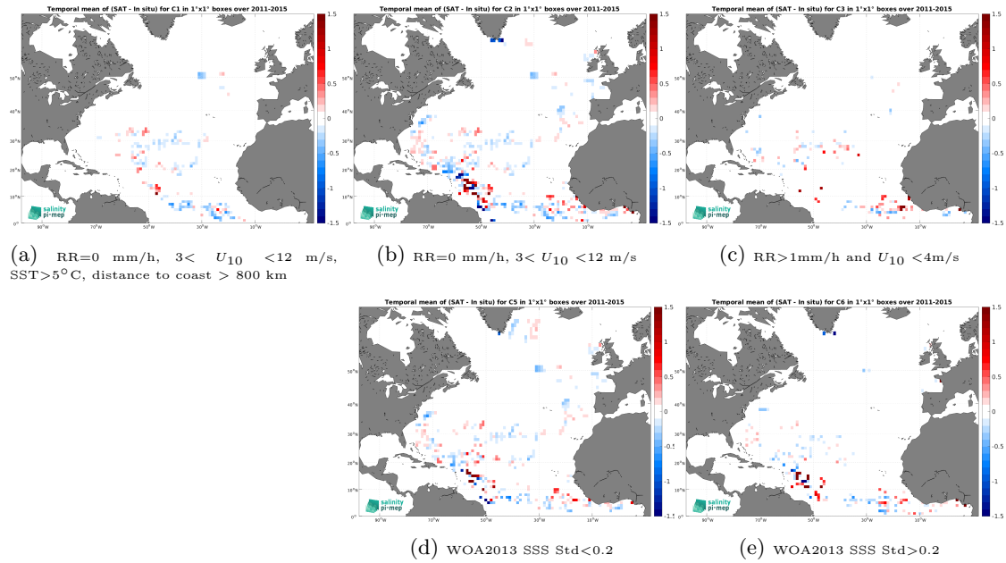
Figure 11: Temporal mean gridded over spatial boxes of size 1^\circ \times 1^\circ of \Delta\text{SSS} (Aquarius SSS L4 OI v5 - Monthly (IPRC) - Surface drifters) for 5 different subdatasets corresponding to:RR=0 mm/h, 3 < U_{10} < 12 m/s, SST >5^\circ\text{C} , distance to coast > 800 km (a), RR=0 mm/h, 3 < U_{10} < 12 m/s (b), RR >1 mm/h and U_{10} < 4 m/s (c), WOA2013 SSS Std <0.2 (d), WOA2013 SSS Std >0.2 (e).
