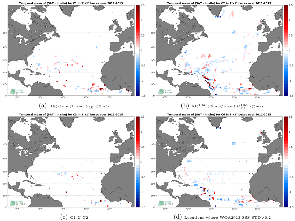
Figure 11: Temporal mean gridded over spatial boxes of size 1^\circ \times 1^\circ of \Delta SSS (Aquarius-L4-IPRC-V5-MONTHLY - Surface drifters) for 4 different subdatasets corresponding to: RR > 1mm/h and U_{10} < 5\text{m/s} (a), RR^{10d} > 5\text{mm/h} and U_{10}^{10d} < 5\text{m/s} (b), C1 U C2 (c), Locations where WOA2013 SSS STD > 0.2 (d).
